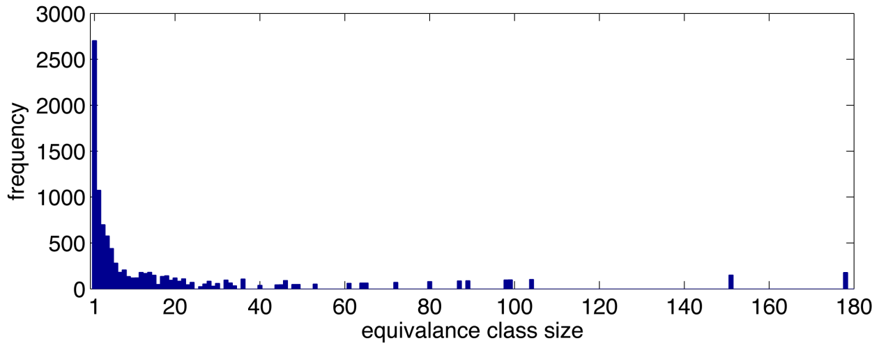
Figure 1: The distribution of equivalence class sizes for paired resolution and JPEG quantization (a class size of 1 denotes a unique pairing).
