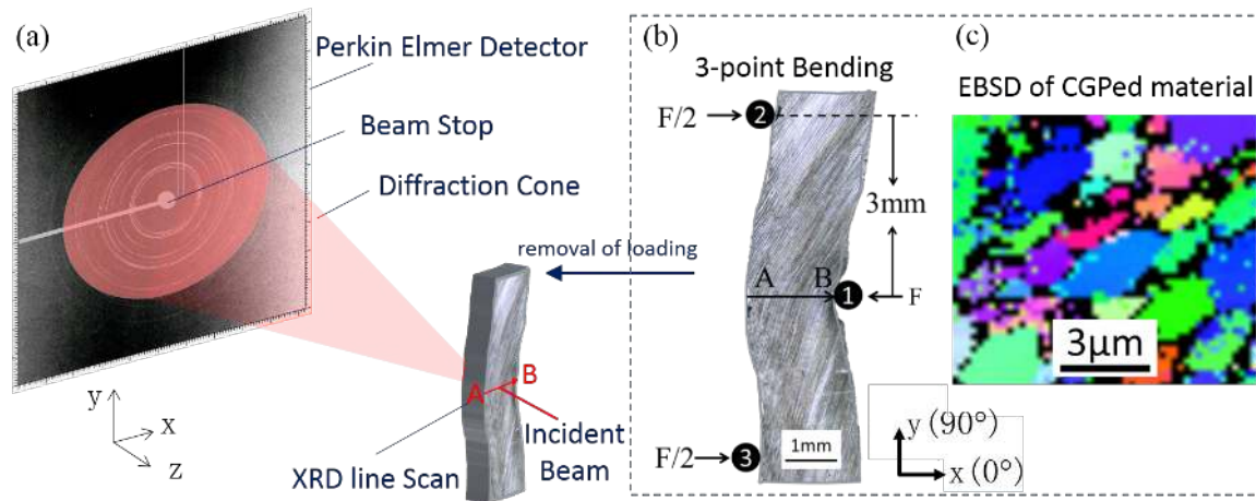
Figure 2. (a) Layout of XRD experiment; (b) Set-up of 3-point bending and (c) EBSD of as-CGPed sample.
