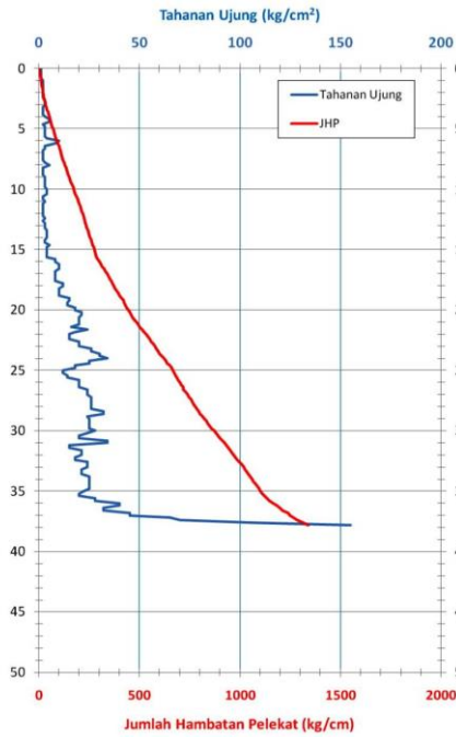
Fig. 2. CPT result of global hotel Banjarmasin.
