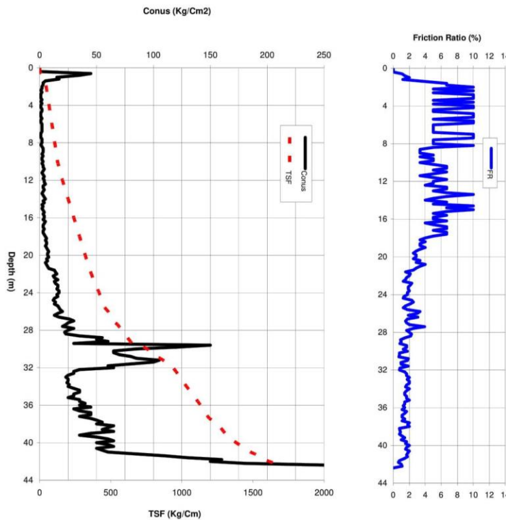
Fig. 4. CPT result of ujung murung street banjarmasin.
