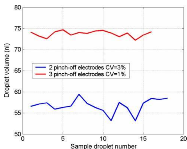
Fig. 22 Dispensed droplet volume control versus the number of serial electrodes interfaced to the reservoir (Ren 2004)
