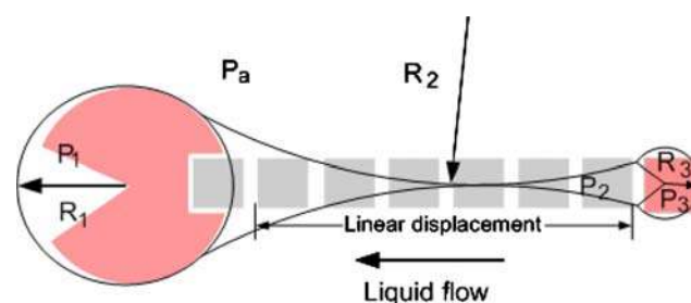
Fig. 18 Breaking of the liquid neck to form a droplet of radius R_3 (Ren et al. 2003a, b)
