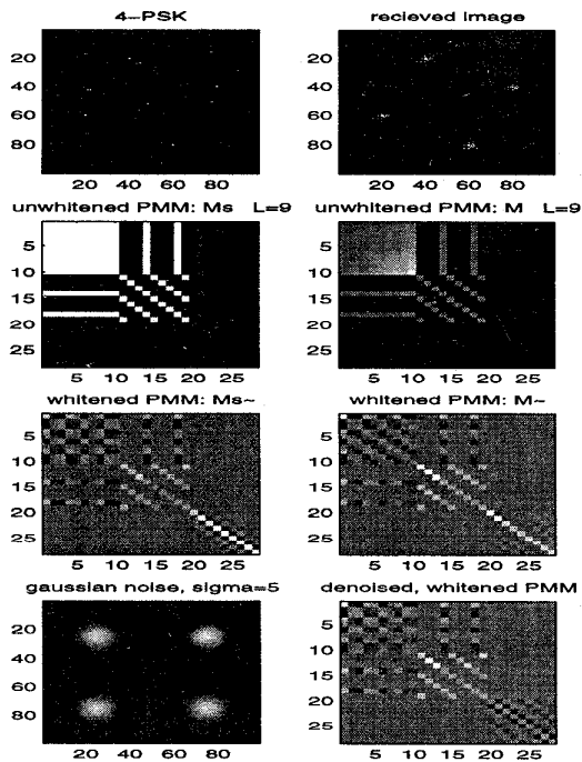
Figure 3: The order of the panels is the same as in figure 2. Note that there is now a mismatch between the noise and the the actual spatial distribution of the received signal. Note further the rotation invariance of PMM.
