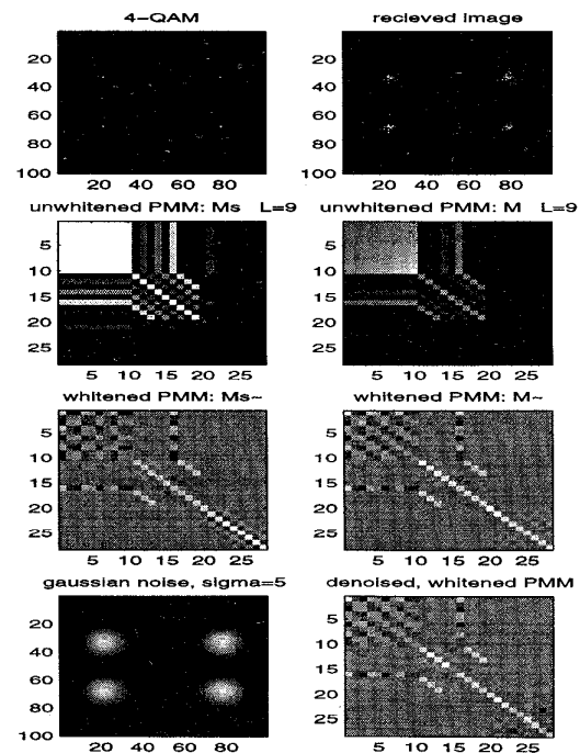
Figure 5: The order of the panels is the same as in figure 4. There is hardly any difference between the moment matrices of figure 4 and the moment matrices in this figure (with the correct cholesky factor).
