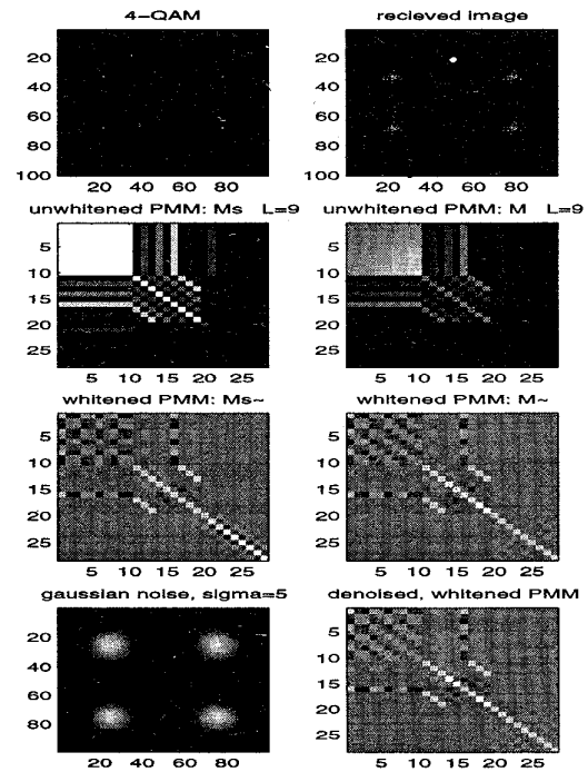
Figure 4: First row: signal alone (left) and noise contaminated IQ images for 4-QAM, second row: unwhitened PMMs, third row: whitened PMMs, fourth row: spatial distribution of the noise(left) and the denoised, whitened PMM. Note that the wrong cholesky factor is used, i.e. the cholesky factor corresponding to 4-PSK.
