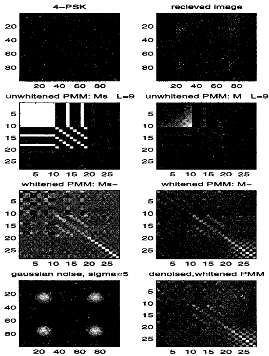
Figure 2: First row: signal alone (left) and noise contaminated IQ images for 4-PSK, second row: unwhitened PMMs, third row: whitened PMMs, fourth row: spatial distribution of the noise(left) and the denoised, whitened PMM.
