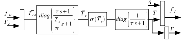
Fig. 5. Relationship between desired inertial control force ( f_{Ic} ) and control torque \Gamma_c to actual inertial force f_I and torque \Gamma .
