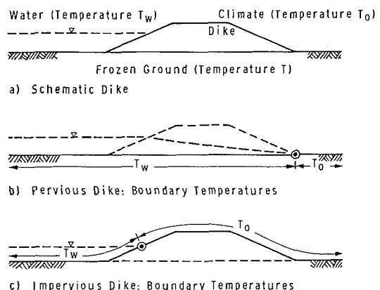
FIG. 1. Dikes on permafrost: thermal considerations.
