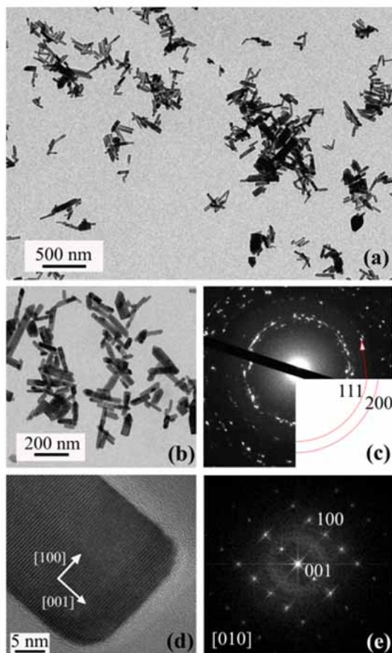
Fig. S1 (a) Overview TEM image of 3% Co:ZnO nanorods; (b) TEM image of 3% Co:ZnO nanorods at higher magnification; (c) Comparison of the SAED pattern of 3% Co:ZnO with the simulated pattern of fcc Co; (d) HRTEM image of a tip of 3% Co:ZnO nanorod with [001] crystal growth direction; (e) Corresponding power spectrum of (d) revealing [010] zone-axis of ZnO.
