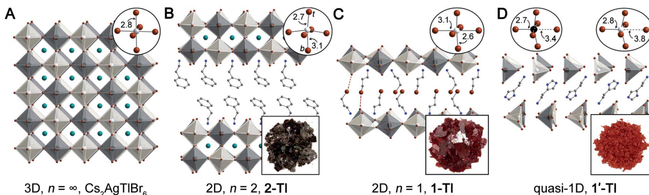
Fig. 1 Single-crystal X-ray diffraction structures of (A) Cs 2 AgTlBr 6 (ref. 5) and three new lower-dimensional derivatives: (B) (PEA) 2 CsAgTlBr 7 ( 2-Tl PEA ; PEA = phenethylammonium), (C) (3-BPA) 4 AgTlBr 8 ( 1-Tl ; 3-BPA = 3-bromopropylammonium) with dotted lines showing Br⋯Br interactions, and (D) (HIS) 2 AgTlBr 8 ( 1'-Tl ; HIS = histammonium). Top insets show the metal coordination spheres ( t = terminal, b = bridging) and bottom insets show the colors of the crystals. Black, white, teal, brown, blue, and gray spheres represent Tl, Ag, Cs, Br, N, and C atoms, respectively. H and disordered atoms omitted for clarity.
