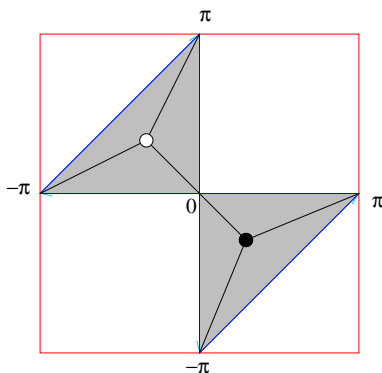
Figure 19: An embedding of the dimer model for \mathbb{C}^3 . The shaded region is the algebra projection of the curve P(z, w) = 1 - z - w = 0 , and in this case it is bounded by the straight-line winding cycles with (p, q) = (1, 1), (-1, 0), (0, -1) .
