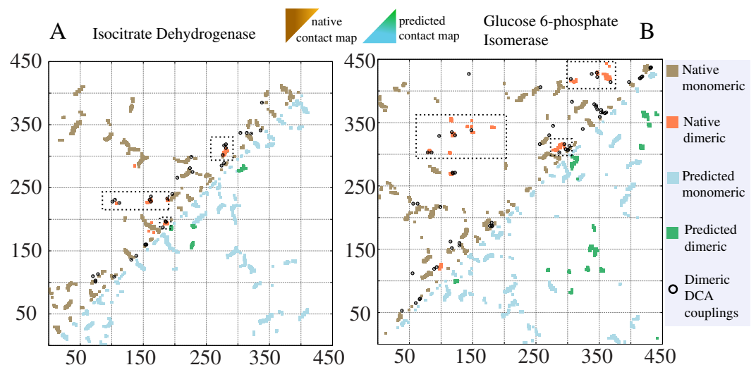
Figure 2. Direct couplings of single domain families contain signals of dimeric interfaces. (A) Contact maps of protein isocitrate dehydrogenase (412 aa). The upper triangular map shows the native monomeric contacts (brown) along with the native dimeric contacts (orange). The circular symbols represent the top ranked couplings estimated using DCA, the solvent accessibility criterion and removing contacts close to the monomeric map. These DCA couplings are used as constrains in the molecular dynamics simulation. The lower triangular map shows the contacts of the best predicted complex obtained after using the SBM + DCA protocol. Monomeric contacts are shown in blue and resulting dimeric contacts in green. (B) Contact maps of glucose 6-phosphate isomerase use the same convention as in (A) with similar and consistent results. The predicted contact maps for the protein-protein interface colored in green are very similar to their native counterparts shown in dashed boxes.
