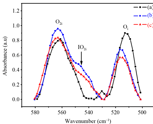
Figure 4. Room temperature IR absorption spectra for: as-grown Si sample (a) heat treated at 450^\circ\text{C} (b) and 800^\circ\text{C} (c) both during 4 h. In this spectral range oxygen dimer formation compete well with the loss of oxygen atoms at high temperatures.
