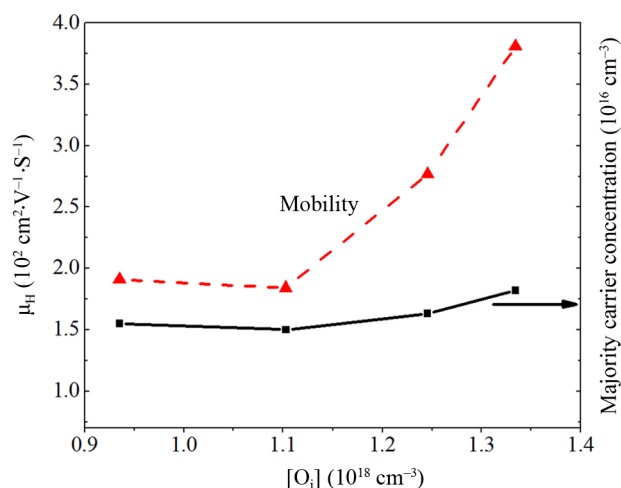
Figure 3. Dependence of the mobility and the majority carrier concentration on interstitial oxygen concentration in boron doped Cz-Si.
