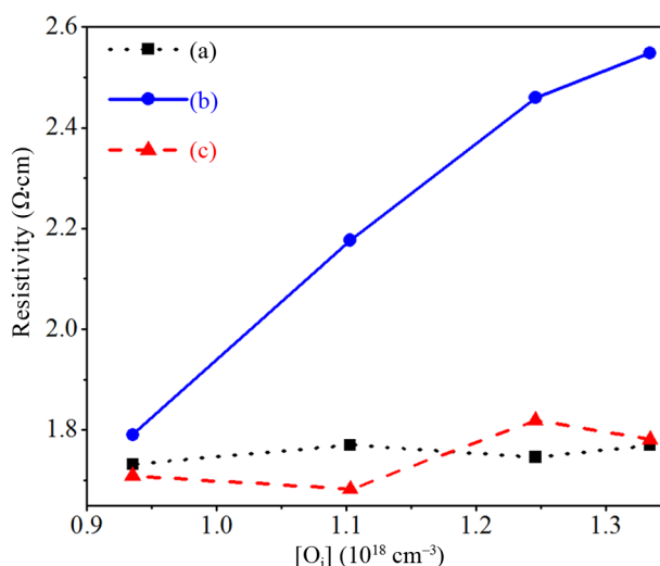
Figure 7. Variation of the resistivity with the concentration of interstitial oxygen for as-grown c-Si wafers (a) after thermal treatment at 450^\circ\text{C} (b) and 800^\circ\text{C} (c) during 4 hours under \text{N}_2 ambient.
