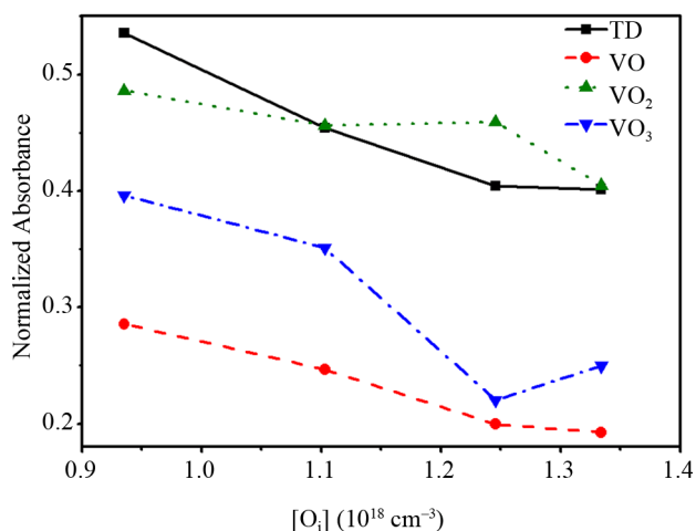
Figure 2. Room temperature FTIR absorbance intensity related to TDs (appearing at 736 \text{cm}^{-1} , squared symbol), VO (circle), VO_2 (up triangle), and VO_3 (down triangle) complexes versus [O_i] in as-grown Cz-Si.
