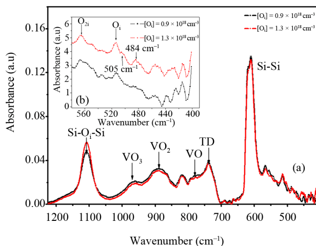
Figure 1. FTIR spectra at 300 K of as-grown Cz-Si samples for [O_i] = 0.9 \times 10^{18} \text{ cm}^{-3} (squared symbol) and [O_i] = 1.3 \times 10^{18} \text{ cm}^{-3} (circle symbol). The discrepancy is induced by the temperature gradient during the cool-down process. The inset shows details of IR bands in the 400 - 600 \text{cm}^{-1} spectral range.
