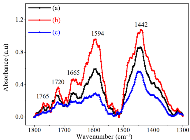
Figure 6. Room temperature absorption spectra of as-grown sample (a) heat treated at 450^\circ\text{C} (b) and subsequently annealed at 800^\circ\text{C} (c) both during 4 h. It shows the relative disappearance of the IR bands at 1665\text{ cm}^{-1} , 1720\text{ cm}^{-1} and 1765\text{ cm}^{-1} upon successive annealing at 800^\circ\text{C} .
