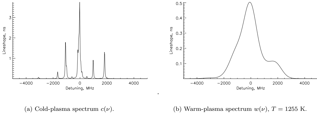
Figure 2. Cold-plasma and warm-plasma spectra for the Xe II 5d^4D_{7/2} - 6p^4P_{5/2}^0 line at 605.1 nm.
