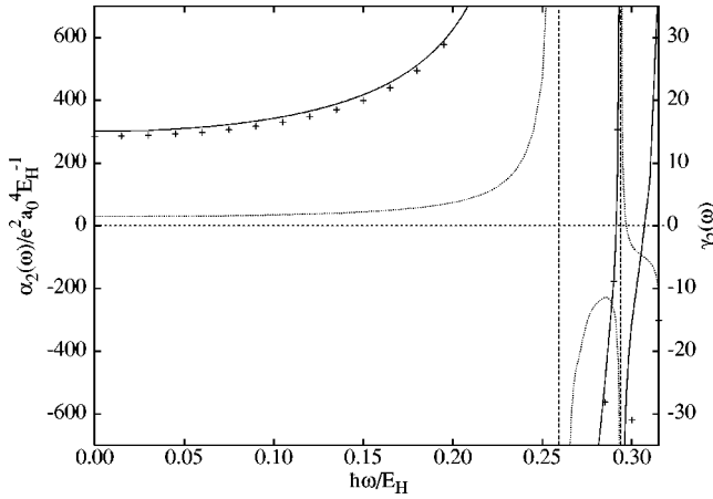
FIG. 4. Dynamic quadrupole polarizability (solid line, left axis) and quadrupole shielding factor (dotted line, right axis) of Be from ECG calculations. 3^1D \leftarrow 2^1S and 4^1D \leftarrow 2^1S transitions are marked at \omega = 0.25916 and \omega_{4^1D} = 0.29375 , respectively. Additionally, results of TDGI calculations of \alpha_2 by Bégué et al. [62] are shown as +.
