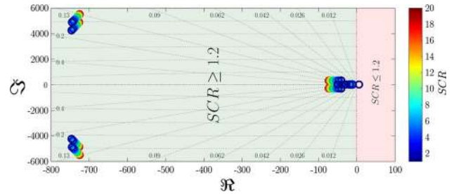
Fig. 9 Impact of the SCR on system stability
