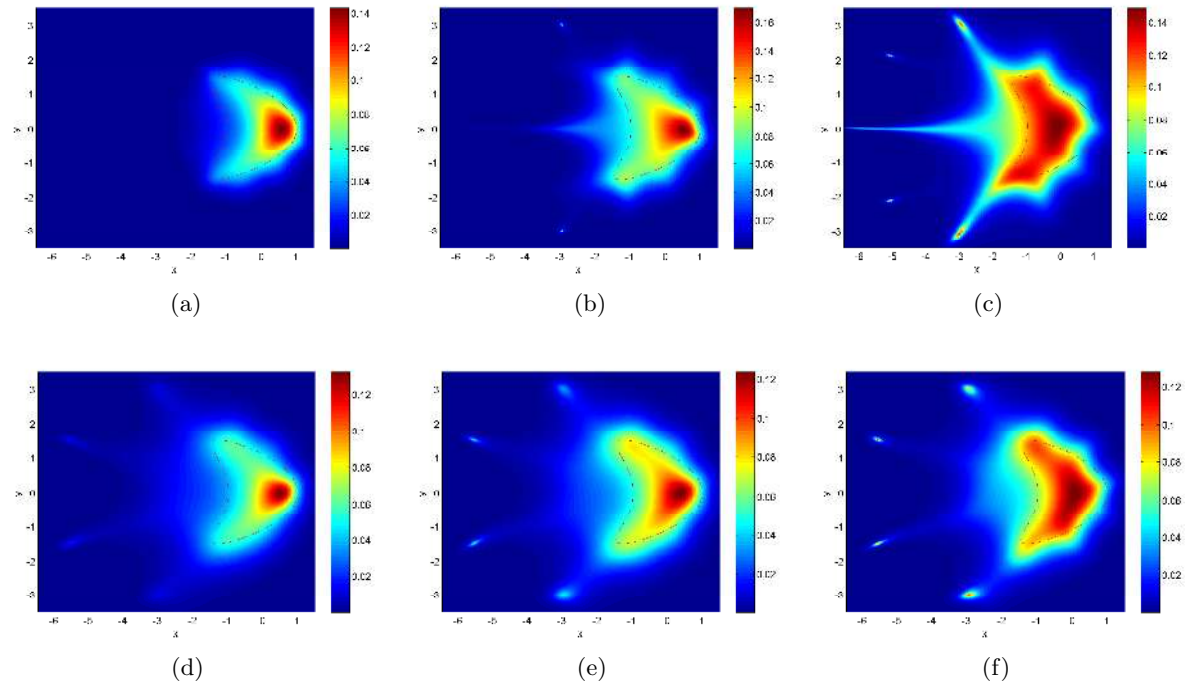
Figure 4: Reconstruction of a kite and N point-like obstacles lying on a half-circle using limited aperture data. In (4a), N = 0 ; In (4b) resp. (4c), N = 3 resp. 5 and \alpha_j = 0.3 . In (4d), (4e) and (4f), we set \alpha_j = 2, 0.75 and 0.3 , respectively and N = 4 .
