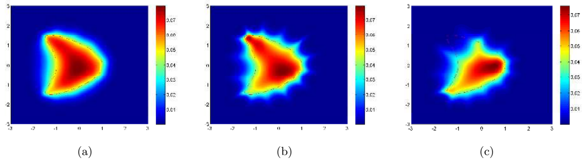
Figure 2: Reconstruction of a kite and one point-like obstacle located at (a, a) . We set a = 8, 4, 1.5 in (2a), (2b) and (2c), respectively.
