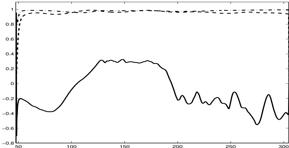
Figure 4.5: Correlation coefficient between -G_1/2 and \mu_{12}/\bar{\rho} \partial_1(\bar{\rho}k) (—), between -G_2/2 and \mu_{12}/\bar{\rho} \partial_2(\bar{\rho}k) (---), and between -G_1/2 and +G_2/2 (-·-) as a function of the streamwise coordinate.
