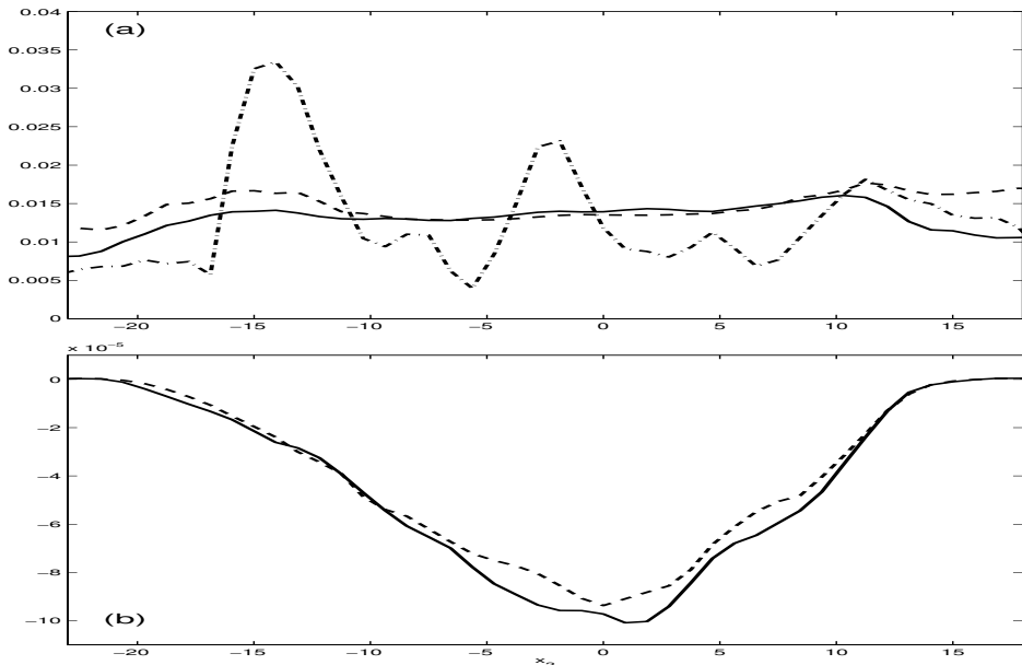
Figure 6.11: Averaged profiles for W (—) and WC_m (-- ) at X_1 = 225 as a function of x_2 . The dynamic coefficient C_m from WC_m is shown together with an instantaneous C_d ( t = 3231 ; ···) and \langle C_d \rangle_t from W in (a). The modeled \langle \bar{\rho}\tau_{12} \rangle is displayed in (b).
