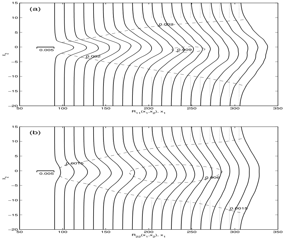
Figure 3.2: Streamwise development of the turbulence intensities R_{11} (a) and R_{22} (b) (—), isolines at 0.002 and 0.009 (a) and 0.0015 and 0.006 (b) (---) and the level of zero ( \cdots ).
