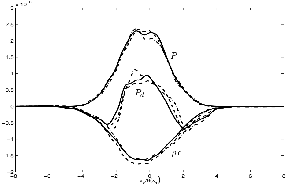
Figure 3.10: Profiles of P , -\bar{\rho}\epsilon and P_d as a function of x_2/\theta(x_1) at x_1 = 241 , normalized with \Delta U^3/\theta(x_1) and averaged over a short (—), middle (---) and long (— · —) time interval (from t = 552 = 25 T_F until T_1 = 70 T_F , T_2 = 110 T_F and T_3 = 150 T_F respectively and based on the fine-grid results).
