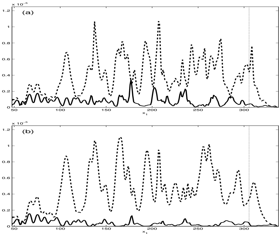
Figure 5.5: Plots of P = -\bar{\rho}\tau_{ij} \partial_j \tilde{u}_i at t = 935 as a function of x_1 and averaged over x_2 and x_3 . The amounts of backscatter |P_-| = -P_- (—) and forward scatter |P_+| = P_+ (---) are shown for the Bardina (a) and dynamic mixed model (b).
