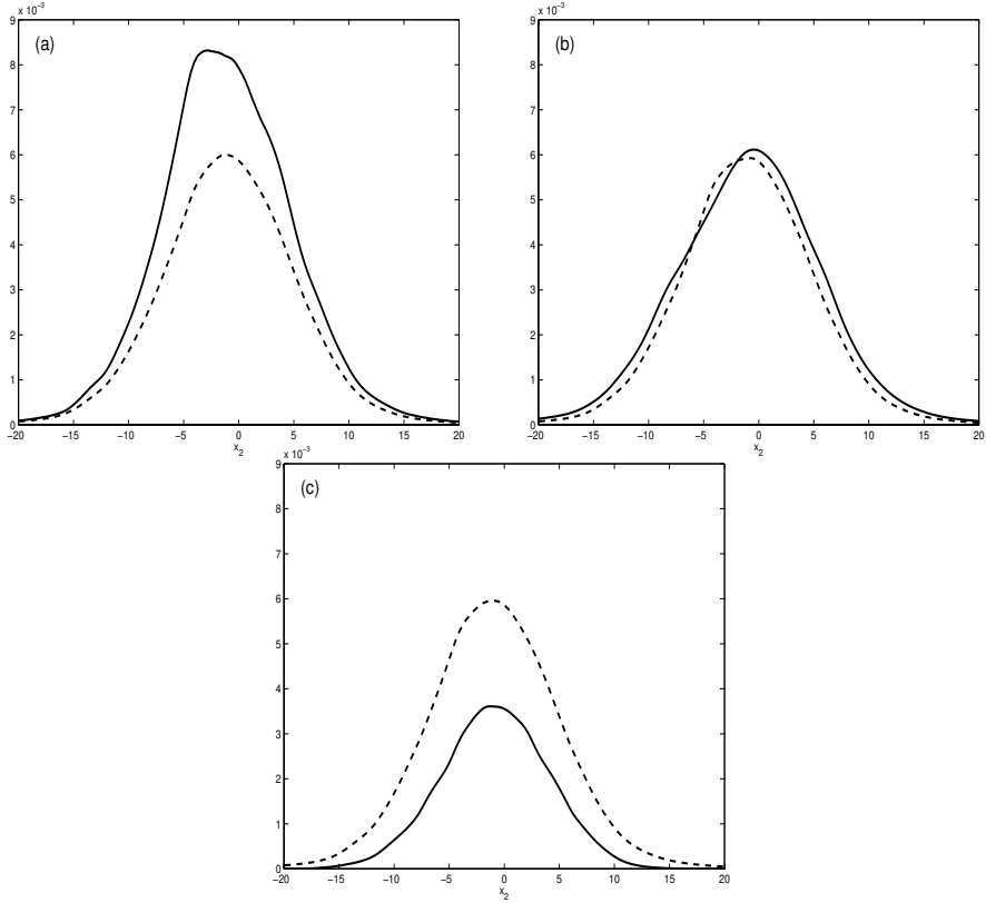
Figure 4.3: Streamwise (a), normal (b) and spanwise (c) turbulence intensities, \overline{\rho u_i'' u_i''} (—), as well as the standard k - \epsilon prediction, -\mu_{k\epsilon}(2\partial_i \tilde{u}_i - 2/3 \partial_k \tilde{u}_k) + 2/3 \bar{\rho} k (---), with i = 1, 2 and 3 at x_1 = 257 as a function of x_2 .
