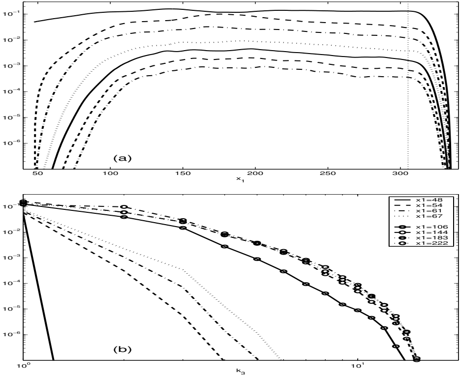
Figure 2.4: Energy spectrum of the reference DNS with LST inflow perturbations. The kinetic energy density E(x_1, k_3) is plotted as a function of x_1 for modes k_3 = 1 (—) to 7 (⋯) (a) and as a function of k_3 for several equidistant streamwise locations: x_1 = 48 (—) to 67 (⋯) and (with symbols) x_1 = 106 (—) to 222 (⋯) (b).
