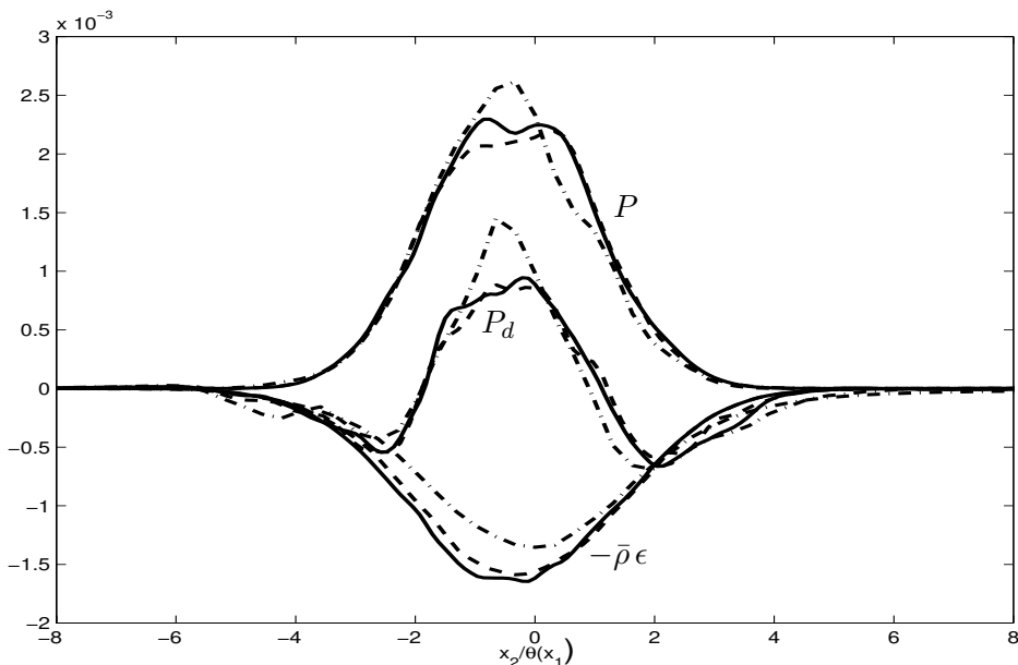
Figure 3.9: Profiles of P , -\bar{\rho}\epsilon and P_d as a function of x_2/\theta(x_1) at x_1 = 241 , normalized with \Delta U^3/\theta(x_1) and plotted for the coarse (---), middle (-.-) and fine (—) resolution DNS (based on the longest time sample available).
