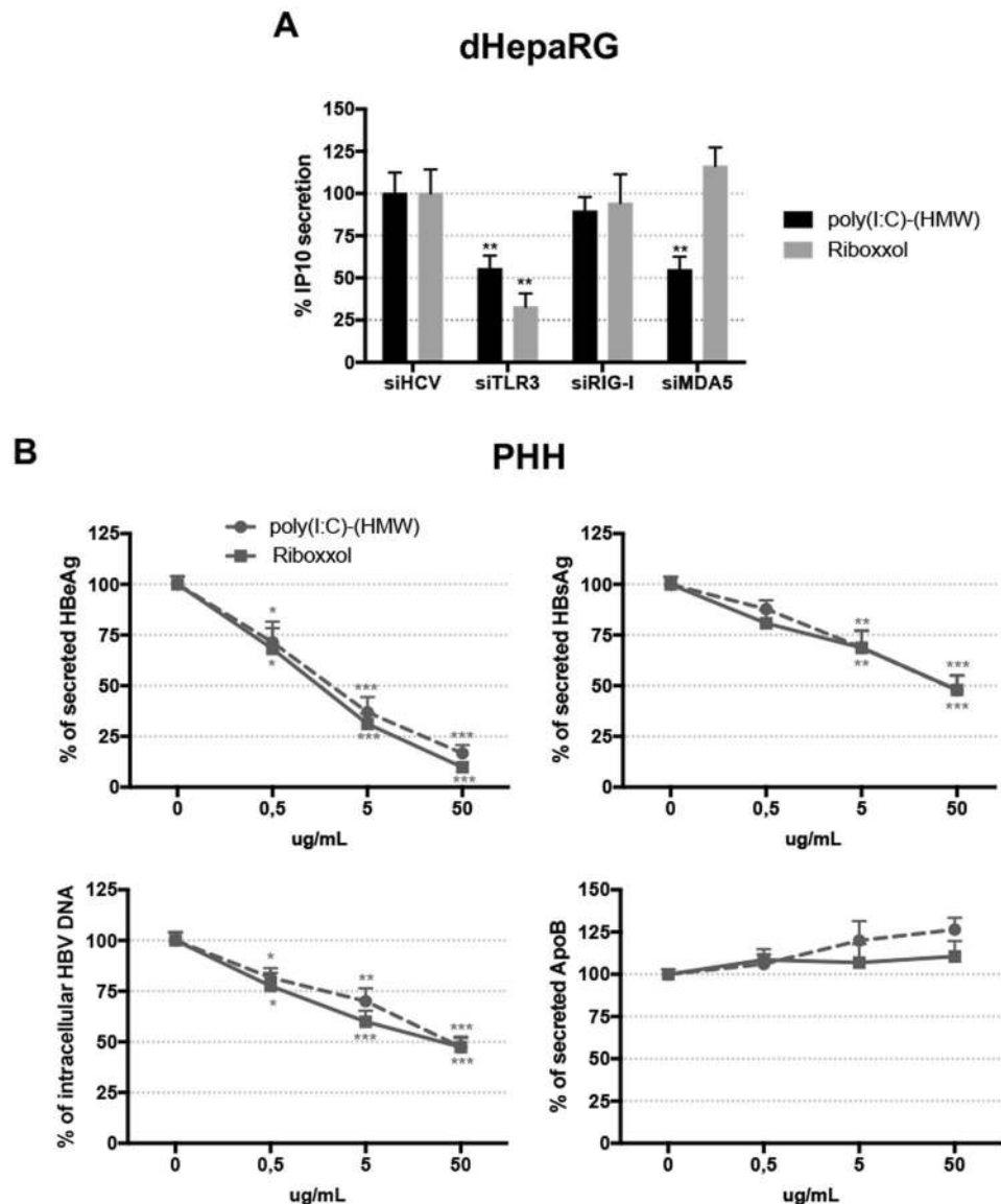
Figure 3. Inhibition of HBV by PolyIC(HMW) and Riboxzol. (A) Uninfected dHepaRG cells were transfected with the indicated siRNA. 14 days later, cells were stimulated with 10 \mu\text{g}/\text{ml} of the indicated ligands. Cells were lysed 24 h later and IP10 secretions were assessed by ELISA. Results are the mean \pm SD of three independent experiments each performed in technical duplicates. (B) PHH were infected by HBV at a multiplicity of infection of 100 viral genome equivalent (vge)/cell for seven days and treated twice with poly(I:C)-(HMW) or Riboxzol at the indicated concentration for seven days. At the end of the experiments, supernatants were collected, and HBeAg, HBsAg and ApoB levels assessed by ELISA. Cells were harvested, total DNAs extracted and total intracellular HBV DNA amounts were quantified by qPCR. Results are the mean \pm SD of four independent experiments (four donors of PHH) each performed with three biological replicates.
