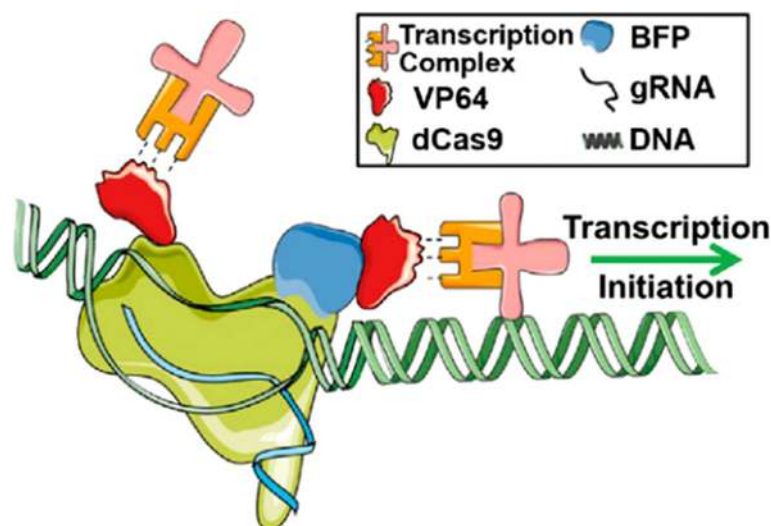
Fig. 2 Schematic of dCas9-VP64. dCas9 binds to the promoter region of the target gene, then uses VP64 to recruit transcription factors to initiate the transcription of the gene [8]
