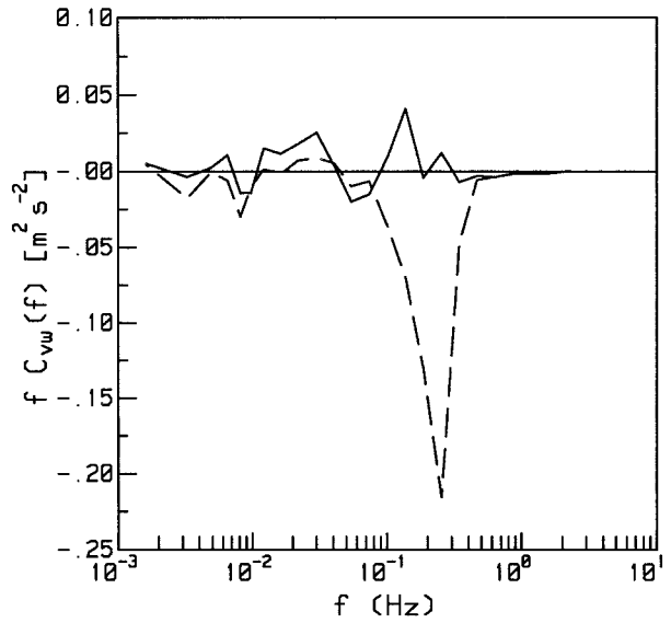
FIG. 8. The uncorrected (broken line) and corrected (solid line) covariance spectra for the lateral component of the momentum flux.
