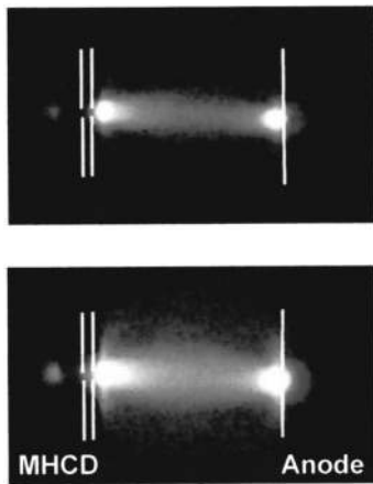
FIG. 2. MCS glow discharge in atmospheric air at two different current levels 8.7 and 22 mA, respectively, at 0.2 cm gap distance. Upper photograph: V_{\text{MHCD}}=499 V, I_{\text{MHCD}}=8.9 mA, V_{\text{MCS}}=250 V, I_{\text{MCS}}=8.7 mA. Lower photograph: V_{\text{MHCD}}=409 V, I_{\text{MHCD}}=27.0 mA, V_{\text{MCS}}=238 V, I_{\text{MCS}}=22.0 mA.
