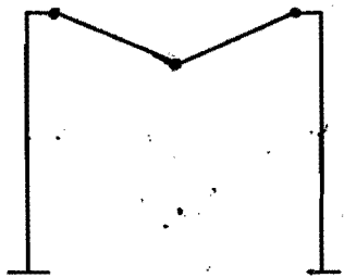
Beam mechanism
