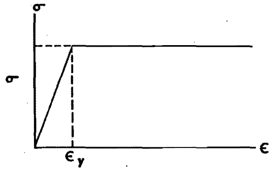
FIG. 2-1 Elasto-plastic stress-strain diagram
