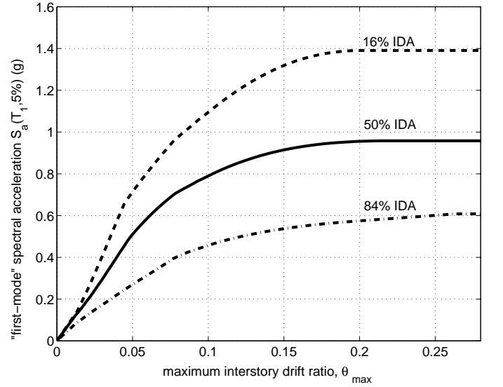
d. SPO2IDA estimated \theta_{\text{max}} fractile curves
