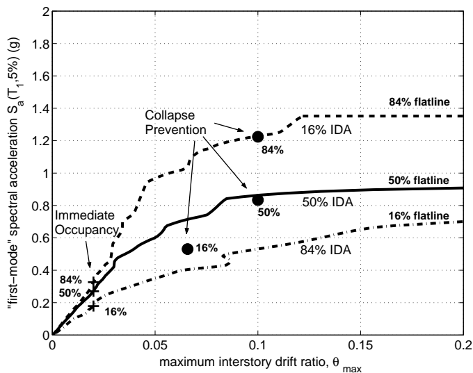
Figure 1. 16%, 50%, 84% fractile IDAs and limit-state capacities
