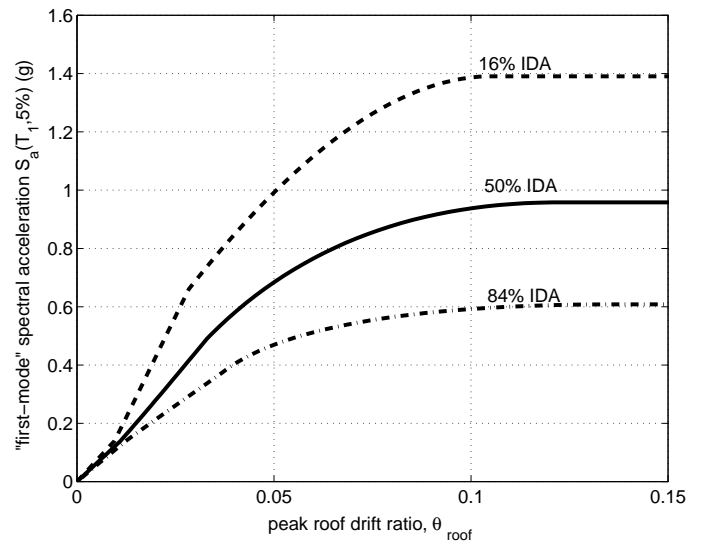
b. SPO2IDA estimated \theta_{\text{roof}} fractile curves
