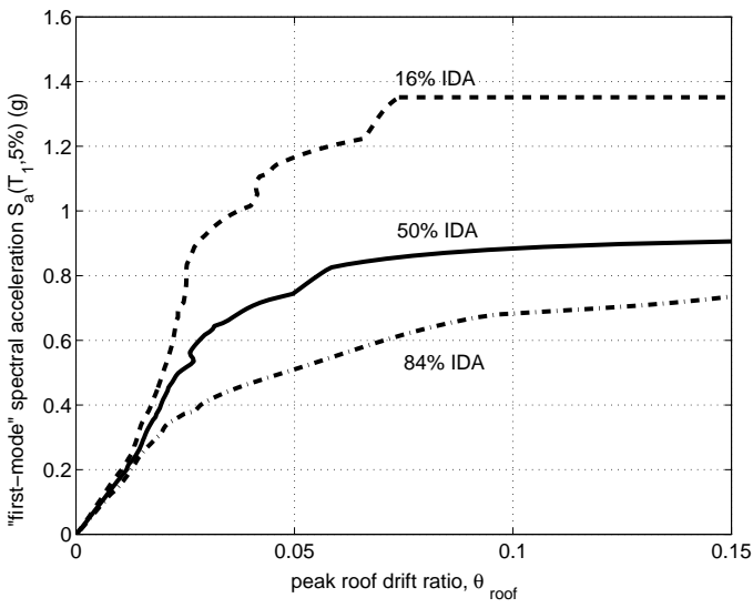
a. Full IDA \theta_{\text{roof}} fractile curves
