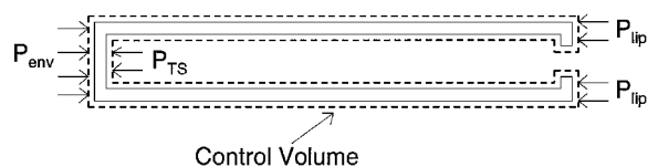
Fig. 1 Pulse detonation engine control volume.
