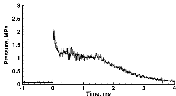
Fig. 3 Sample pressure trace of stoichiometric \text{C}_2\text{H}_4\text{-O}_2 at 100-kPa initial pressure recorded at the thrust surface.
