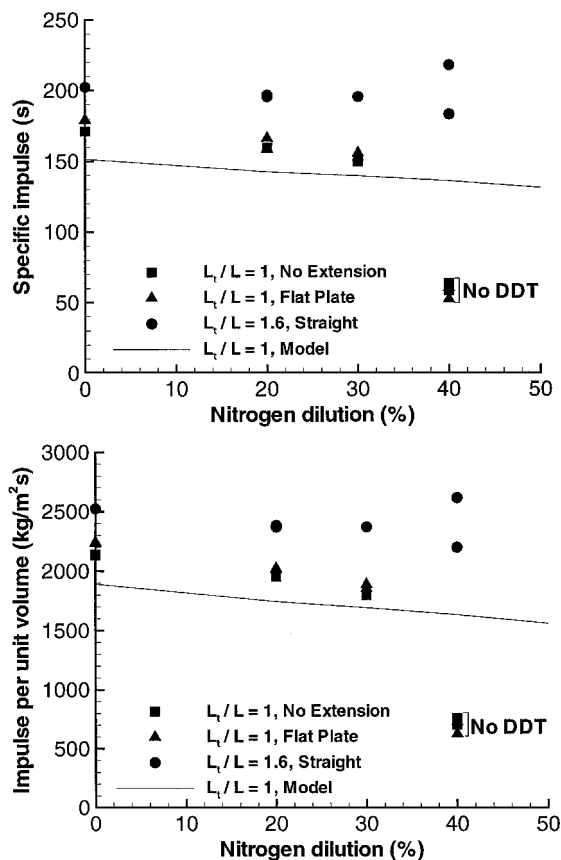
Fig. 17 Specific impulse for stoichiometric C_2H_4-O_2 mixtures at 100-kPa initial pressure with varying diluent and no internal obstacles.
