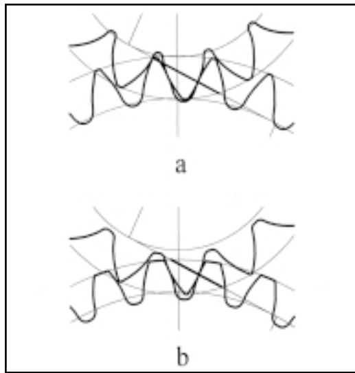
Figure 7 —Involute meshes for the gear pair z_1 = 14 , z_2 = 28 (at point E of the area of existence shown in Figure 5, \alpha_w = 25^\circ ) 7a, direct designed gears ( \epsilon_\alpha = 1.47 ); 7b, standard designed gears ( \epsilon_\alpha = 1.16 ).
