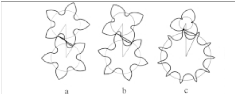
Figure 10—Spur gears with minimum number of teeth: a) z_1 = 5, z_2 = 5, \alpha_w = 33.1^\circ, \epsilon_{\alpha} = 1.04 ; b) z_1 = 4, z_2 = 6, \alpha_w = 32.6^\circ, \epsilon_{\alpha} = 1.02 ; c) z_1 = 3, z_2 = 11, \alpha_w = 24.3^\circ, \epsilon_{\alpha} = 1.01 .
