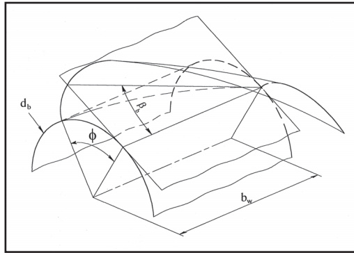
Figure 4—The angular shift of the transverse sections for a helical gear.
