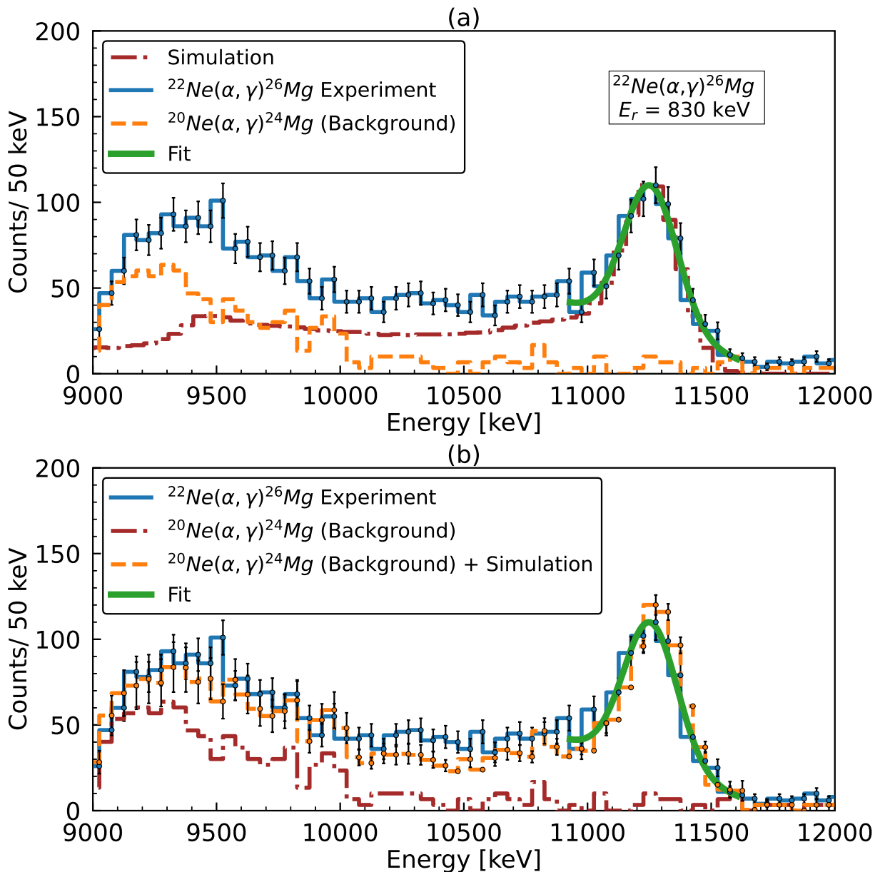
FIG. 5. (a) Sum spectra for the E_{\alpha}^{lab} = 830 \text{ keV} resonance. The solid (blue) histogram shows the sum spectrum from the ^{22}\text{Ne}(\alpha, \gamma)^{26}\text{Mg} reaction and the sum peak is located at E_{\Sigma} = E_{CM} + Q = 11.3 \text{ MeV} . The dashed (orange) histogram shows the beam induced background using the ^{20}\text{Ne} target. The dash dotted (brown) histogram shows the simulated spectrum obtained from GEANT4 [22]. The thick solid (green) line shows the Gaussian plus a linear function fit to the sum peak. (b) The dashed (orange) histogram is the sum of beam induced background and simulation. It shows excellent agreement with the experimental spectrum shown in solid (blue).
