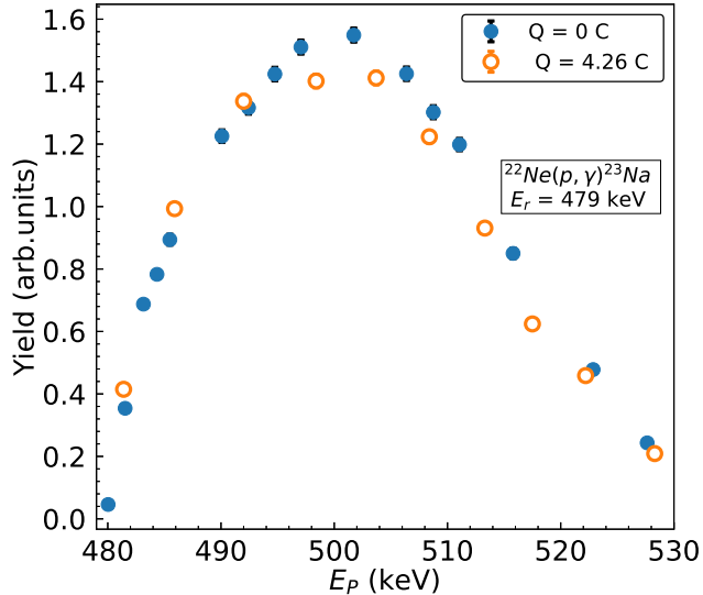
FIG. 4. Yield curve for the E_P^{lab} = 479 keV resonance in the ^{22}\text{Ne}(p, \gamma)^{23}\text{Na} reaction. The yield curve is obtained from the sum peak in HECTOR [19]. The filled-circle (blue) and open-circle (orange) data points show the difference in yield at the beginning and at end of the experiment. The statistical error in the data is \simeq 1\% , which is why the error bars are not visible.
