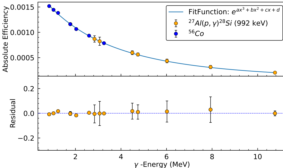
FIG. 1. Absolute \gamma -ray detection efficiency as a function of energy for the Ge detector used for the determination of target stoichiometry.
