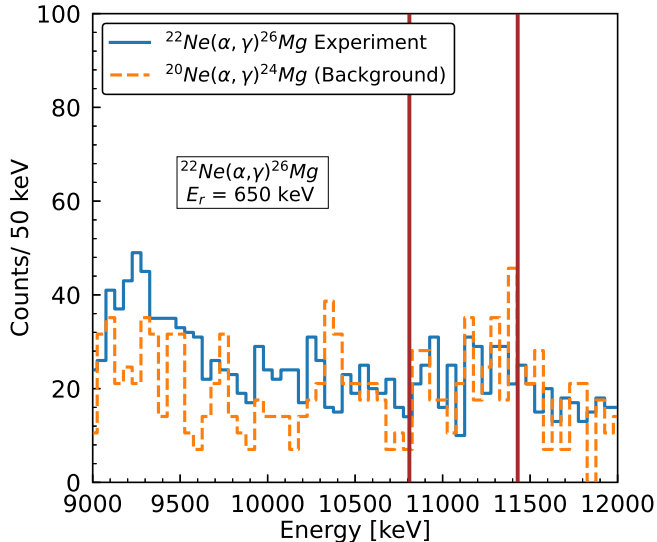
FIG. 6. Sum spectra for the E_{\alpha}^{lab} = 650 keV resonance. The solid (blue) histogram depicts the sum spectrum from the ^{22}\text{Ne}(\alpha, \gamma)^{26}\text{Mg} reaction, whereas the dashed (orange) histogram shows the beam induced background using the ^{20}\text{Ne} target. The two solid vertical lines show the region of integration for the sum peak. The background (orange) histogram was normalized to the same accumulated charge.
