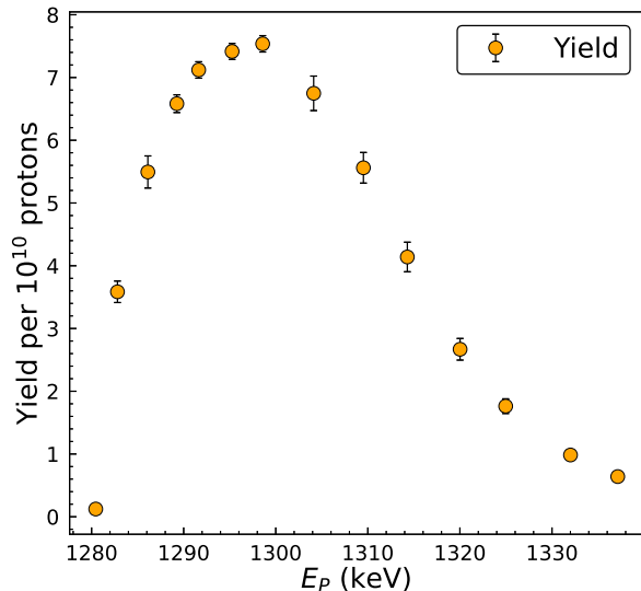
FIG. 2. Yield curve for the E_p^{\text{lab}} = 1278 keV resonance in the ^{22}\text{Ne}(p, \gamma)^{23}\text{Na} reaction.
