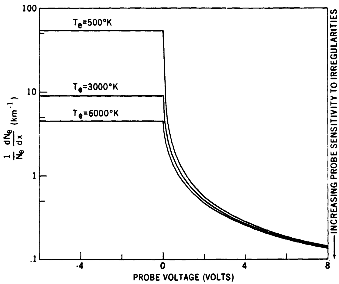
Figure 11a—Minimum electron density gradients required to produce detectable fine structure. N_e gradients are detected more readily in the electron saturation region of the ampere-volt curve.
