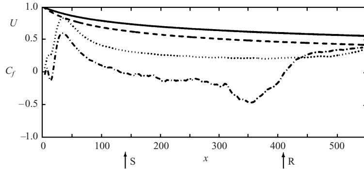
FIGURE 4. APG1: —, U ; \cdots , C_f \times 100 . SEP: ----, U ; -·-·-, C_f \times 100 . S and R denotes point of separation and reattachment respectively for SEP.
