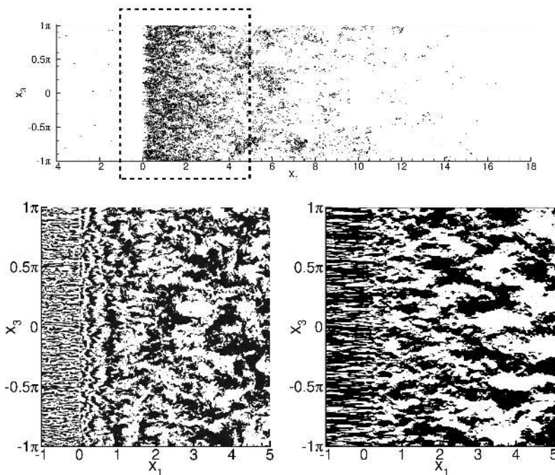
FIGURE 16. A slice parallel to the lower wall at x_2^+ = 1 showing instantaneous views of the Q -invariant (top), u_2' (bottom-left) and u_1' (bottom-right). Black zones denote the highest values of the Q -invariant at the top figure and positive values at the bottom ones.
