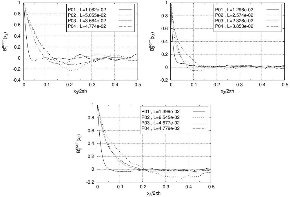
FIGURE 4. Two-point correlation in the span-wise direction of three velocity components at P01, P02, P03 and P04 location (see figure 1). The integral scale value ( L ) of each cross-correlation is presented at the legend. Stream-wise (top-left), Normal (top-right) and Span-wise (bottom) components.
