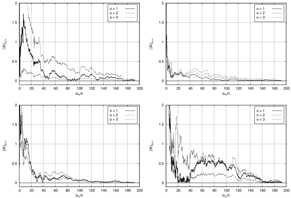
FIGURE 3. Normalized infinite norm ( \|A\|_{\infty} ) (defined in Eq.3.1) of the 1 st , 2 nd and 3 rd order of the non-zero velocity turbulent statistic at P01(top-left), P02 (top-right), P03 (bottom-left) and P04 (bottom-right). Probes location is defined in figure 1.
