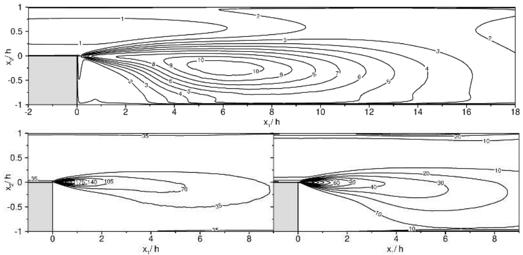
FIGURE 13. Reynolds stress \langle u'_3 u'_3 \rangle / u_\tau^2 (top) and their associated transport source-sink terms scaled using u_\tau^3/h : pressure-strain \langle \Pi_{33} \rangle (left-bottom) and dissipation \langle \varepsilon_{33} \rangle (right-bottom). Dashed lines depict negative values.
