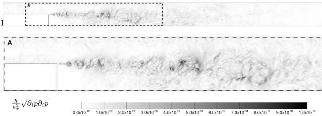
FIGURE 15. Instantaneous magnitude of the dimensionless pressure gradient in a large part of the BFS domain (top), and a detailed view (A) of the sudden expansion (bottom). The colour meaning can be observed in the gray scale. See the film attached in the paper data base (Pont-Vílchez et al. 2018).
