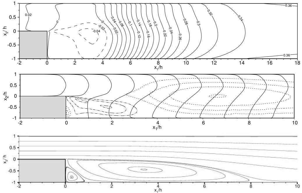
FIGURE 7. Pressure coefficient distribution (top), \langle C_p \rangle , the average velocity field (centre), \langle u_i \rangle , and flow streamlines in the recirculation region (bottom). For the sake of clarity, the stream-wise velocity, \langle u_1 \rangle , is referred using solid lines, whereas the normal velocity component, \langle u_2 \rangle , is depicted using isolines (where dashed lines denote positive values and dot-dashed lines denote negative ones). The \langle u_1 \rangle values have been normalized using the maximum velocity at each profile, following the Ötügen (1991) criterion.
