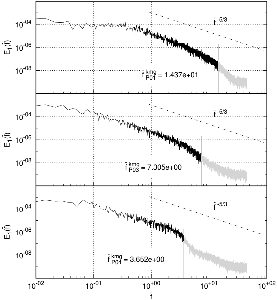
FIGURE 17. Normalized turbulent kinetic energy ( E_1 ) vs normalized temporal frequency ( \bar{f} = fh/U_b ) at P01 (top), P03 (centre) and P04 (bottom). The dashed lines represent the expected turbulence decayment behaviour at the inertial region ( \bar{f}^{-5/3} ), whereas \bar{f}_{P0N}^{kmg} denotes the local Kolmogorov temporal frequency in probe N .
