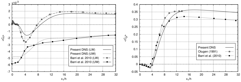
FIGURE 8. Comparison of the skin friction (left), \langle C_f \rangle , at Re_\tau = 395 (present DNS) with the results obtained by Barri et al. (2010) at Re_\tau = 180 using an ER = 2 . The \langle C_f \rangle is assessed in the lower ( LW ) and upper ( UW ) walls. Pressure coefficient (right), \langle C_p \rangle , at the LW obtained in the present DNS compared to the results provided by Barri et al. (2010), Re_\tau = 180 , and Ötügen (1991), Re_\tau = 395 .
