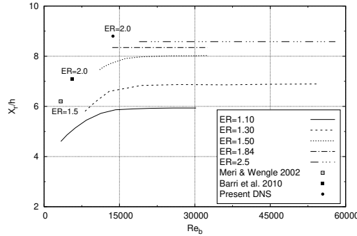
FIGURE 9. Recirculation length ( X_r ) using different Reynolds ( Re_b ) and expansion ratios ( ER ). Experimental results depicted by lines were obtained by Nadge & Govardhan (2014).
