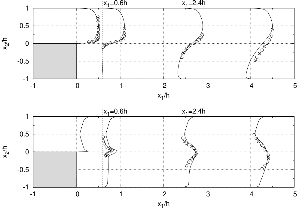
FIGURE 10. Stream-wise velocity (top) and rms (bottom) profiles of the present DNS (—) compared to the experimental results (○) obtained by Ötügen (1991). Velocity ( u_1 ) and rms are normalized using the maximum value at each profile, U_c .
