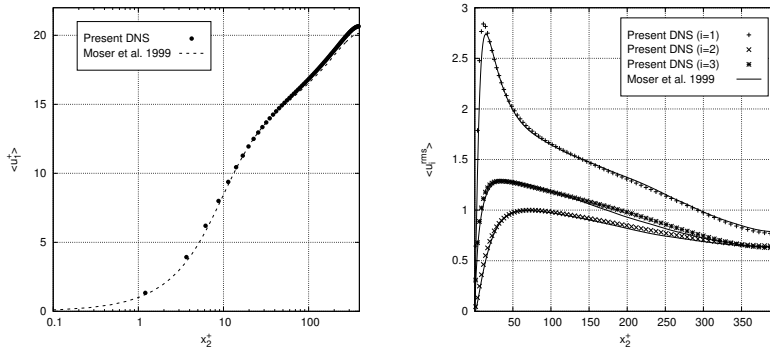
FIGURE 2. Log-Law (left) and Root-Mean-Square (right) profiles at -5h over the step ( 1h downstream of the inflow). Moser et al. (1999) results are used as benchmark data.
