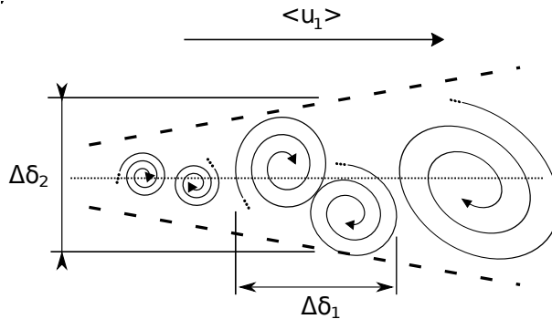
FIGURE 18. Schematic view of the Kelvin-Helmholtz vortices in a shear layer, where \Delta\delta_1 and \Delta\delta_2 represent an estimation of the vortex size in the stream-wise and normal direction, respectively.
