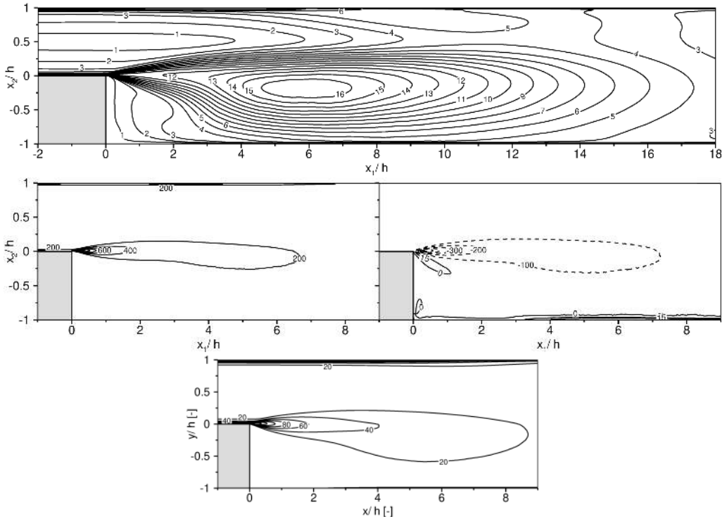
FIGURE 11. Reynolds stress \langle u'_1 u'_1 \rangle / u_\tau^2 (top) and their associated transport source-sink terms scaled using u_\tau^3/h : production \langle P_{11} \rangle (middle-left), pressure-strain \langle \Pi_{11} \rangle (middle-right) and dissipation \langle \varepsilon_{11} \rangle (bottom). Dashed lines depict negative values.
