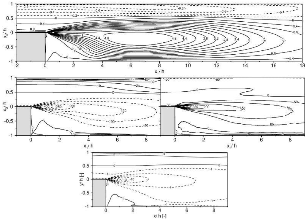
FIGURE 14. Reynolds stress -\langle u_1 u_2' \rangle / u_\tau^2 (top) and their associated transport source-sink terms scaled using u_\tau^3/h : production \langle P_{12} \rangle (middle-left), pressure-strain \langle \Pi_{12} \rangle (middle-right) and dissipation \langle \varepsilon_{12} \rangle (bottom). Dashed lines depict negative values.
