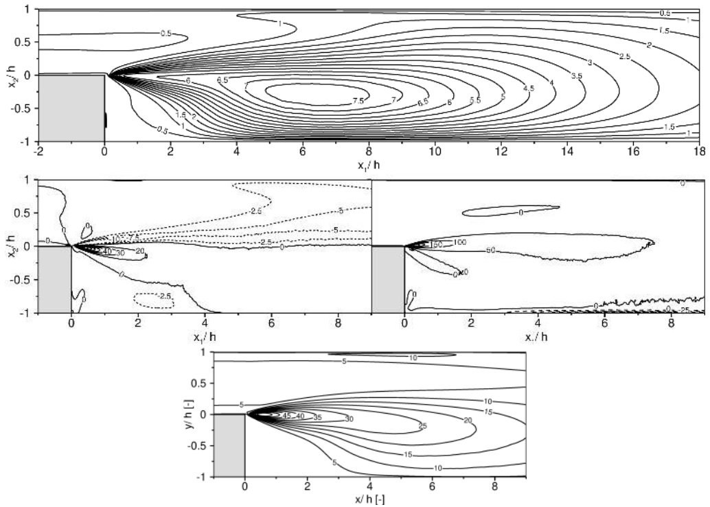
FIGURE 12. Reynolds stress \langle u'_2 u'_2 \rangle / u_\tau^2 (top) and their associated transport source-sink terms scaled using u_\tau^3/h : production \langle P_{22} \rangle (middle-left), pressure-strain \langle \Pi_{22} \rangle (middle-right) and dissipation \langle \varepsilon_{22} \rangle (bottom). Dashed lines depict negative values.
