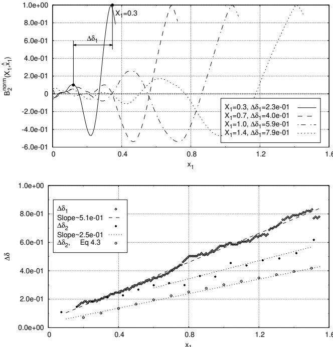
FIGURE 19. An example showing how \Delta\delta_1 have been assessed using two-point correlation at the shear layer (top). Estimation of the KH rate of growth ( \Delta\delta_1, \Delta\delta_2 ) along the stream-wise direction (bottom), which is schematically depicted in figure 18.
