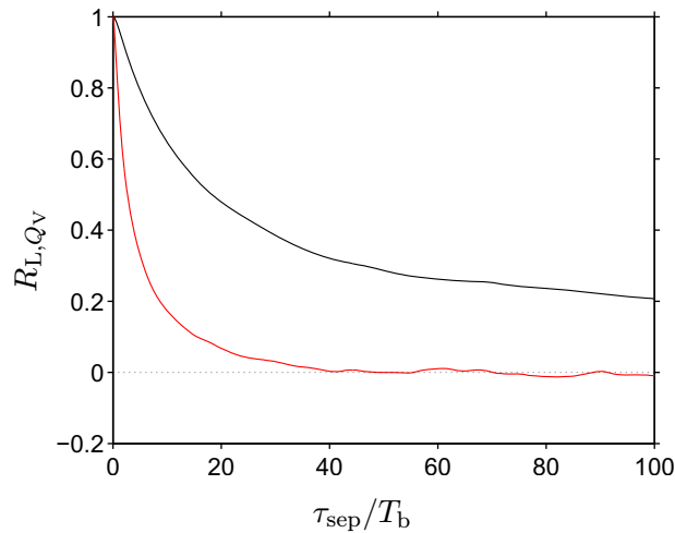
Figure 17. Lagrangian autocorrelation as a function of time lag \tau_{sep} for the Voronoi area (—) and the Voronoi cell aspect ratio (—).
