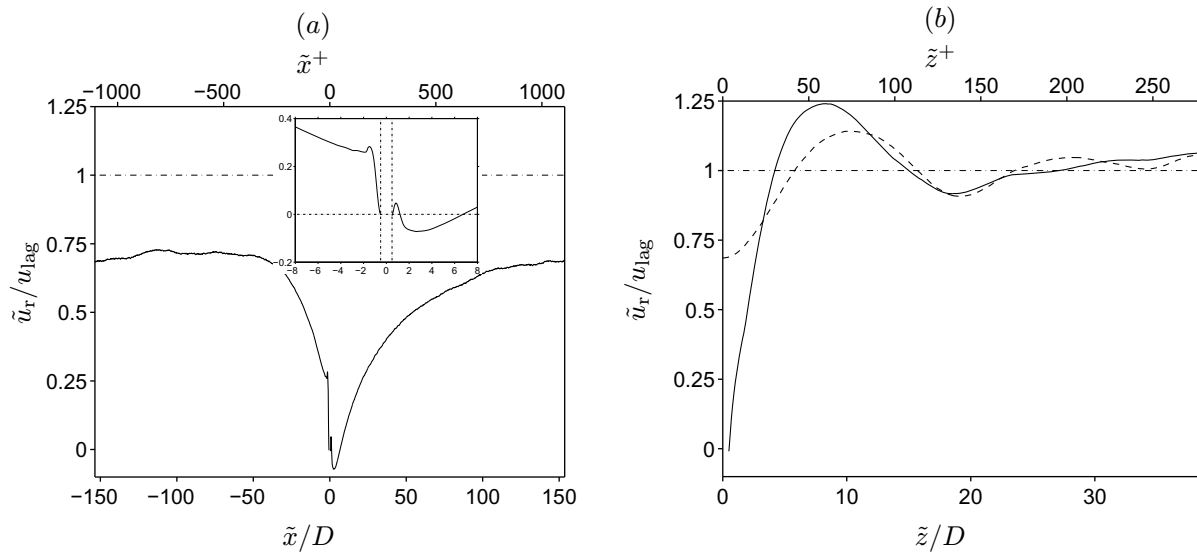
Figure 21. The same quantity \tilde{u}_r / u_{\text{lag}} as in figure 20. Panel (a) shows a streamwise profile through the particle centre ( \tilde{z} = 0 ), with the inset presenting a zoom around the particle location. Panel (b) shows spanwise profiles through the particle centre at \tilde{x} = 0 (solid line) and at \tilde{x} = 6h (dashed line). Note that the data in (b) are symmetric with respect to \tilde{z} = 0 .
