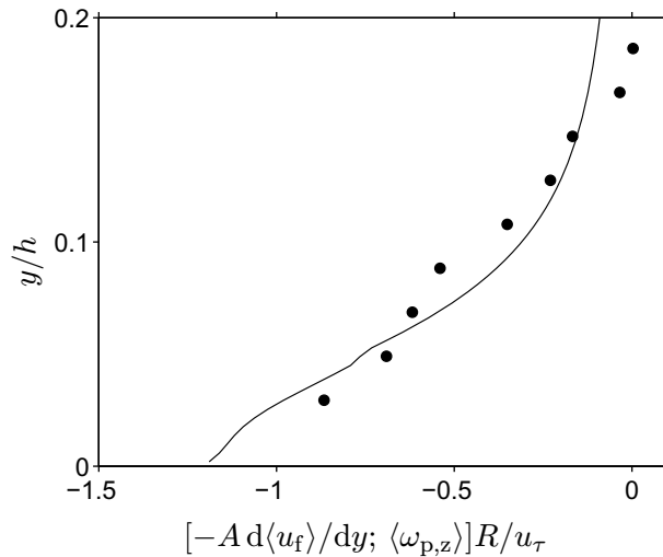
Figure 9. Wall-normal profiles of the mean fluid shear (solid line) and mean value of the spanwise component of particle angular velocity (symbols). The proportionality factor is given as A = 0.33 .
