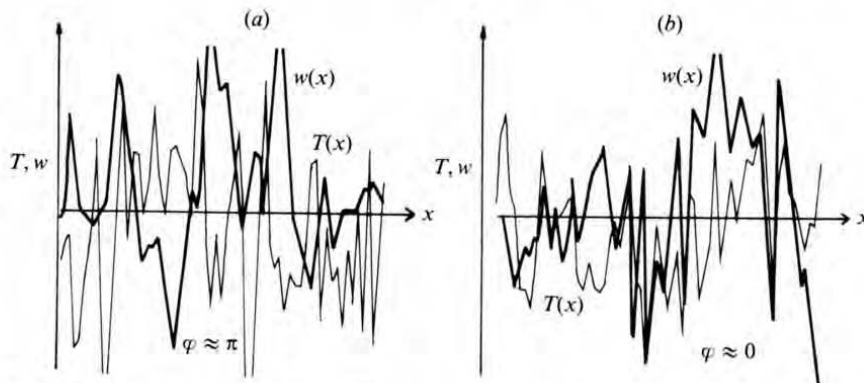
FIGURE 10. Instantaneous velocity and temperature signals versus downstream coordinate x as computed for t = 4 , and y = 0.5, z = 0 with (a) Ri = 0 and (b) Ri = 1 . The signals show the expected phase angles.
