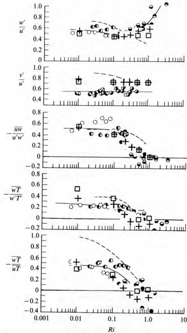
FIGURE 5. Turbulence quantities versus gradient Richardson number. The experimental data of Komori et al. (1983) in water are shown by circles ( \circ , \ominus , \bullet ) and by approximate interpolation (full curve). The dashed curve represents Webster's (1964) measurements in air. The simulation results are indicated by crosses (+) for Pr = 5 , and by squares ( \square ) for Pr = 0.7 at t = 4.5 .
