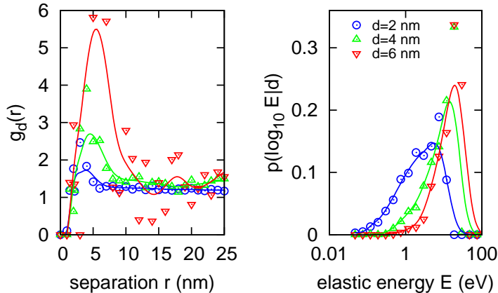
Figure 5: Analysis of spatial correlations of defect clusters obtained from micrographs of 400 keV W^+ irradiated tungsten at 30 K. (a) The radial pair distribution function g_d(r) is plotted against the separation distance r for defects with diameters d > 0, 2, 4, 6 nm. The solid lines are to guide the eye. (b) A characteristic elastic energy scale computed from the size and estimated separation of the loops (see text).
