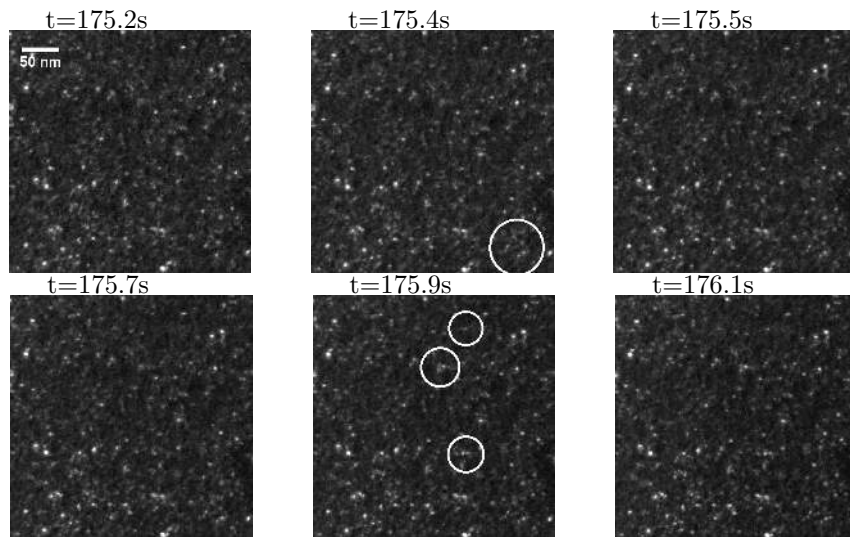
Figure 1: A sequence of snapshots taken over 1s irradiation with 400keV ions showing the space- and time- correlated appearance of nano-scale defects. Contrary to the case in iron, where the defects produced at low fluence are very small[6], individual cascade events in tungsten produce correlated clusters of defects up to 9nm diameter, which appear at full brightness in a single frame and then do not subsequently evolve.
