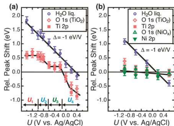
Fig. 3 (a) AP-XPS peak positions of O 1s and Ti 2p 3/2 signals for liquid water and TiO 2 as a function of the potential, U , of a bare p^+ -Si/TiO 2 electrode in 1.0 M KOH(aq). Different potential regions U_1 to U_4 are shown. A solid line corresponding to a slope of \Delta = -1 eV V -1 has been drawn through the water O 1s data; a solid line drawn as a visual guide is shown for the titania data. (b) Analogous AP-XPS peak positions vs. electrode potential for a p^+ -Si/TiO 2 /Ni (deposited by 60 s of Ni sputtering) electrode.
