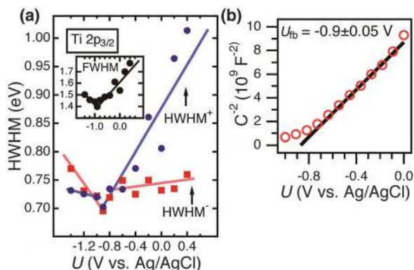
Fig. 5 (a) High and low energy half widths at half maximum (HWHM + , HWHM - ) for the Ti 2p 3/2 peak of a p + -Si/ \text{TiO}_2 electrode as a function of applied potential. The higher binding energy half width, HWHM + , is shown in blue and the lower binding energy half width, HWHM - , in red. The inset depicts the overall full width at half maximum (FWHM = HWHM + + HWHM - ) as a function of applied potential. The blue, red, and black lines are guide-lines for the eye. Error bars are \pm 0.1 eV for the half widths; while the error bars are considerably larger than the trends at negative potentials, the data confirms that the width of the peak increases with an absolute value of U as expected from theoretical simulation. (b) Mott-Schottky data for a p + -Si/ \text{TiO}_2 electrode, with U_{\text{fb}} calculated as -0.9 V vs. Ag/AgCl from a linear fit; a Randles circuit was used as the equivalent circuit.
