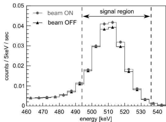
FIG. 3 (color online). Energy spectra of the LaBr 3 (Ce) scintillator in the highest power on-resonance run (run I, 11.0_{-3.3}^{+3.6} kW) after all event selections are applied. Circles and triangles show beam ON and beam OFF spectra, respectively.
