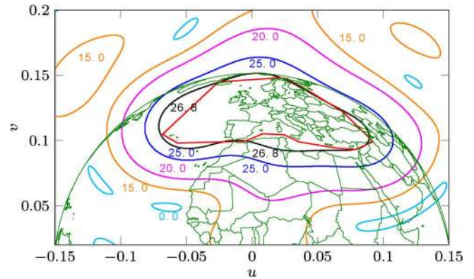
Fig. 3. Simulated co-polar radiation patterns of Design A-II at 10 GHz.
