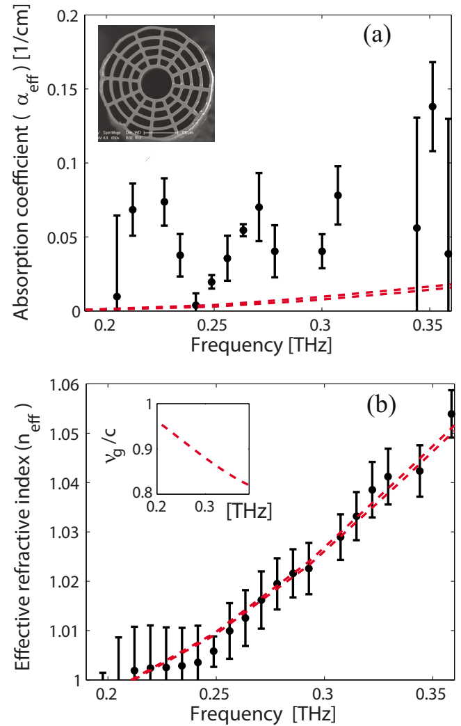
FIG. 2. (Color online) (a) Absorption coefficient, \alpha_{\text{eff}} , and (b) effective refractive index of the propagating fundamental mode in a 600 \mu\text{m} COC spider-web porous fiber: black dots and red dashed lines represent the measured and theoretical values, respectively. The fiber cross-section and group velocity are shown in the inset of parts (a) and (b), respectively.
