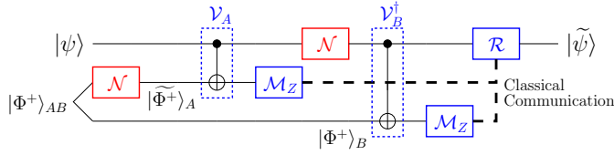
Fig. 3: The quantum circuit conceived for performing a single-qubit error-detection using a single noisy EPR pair.
