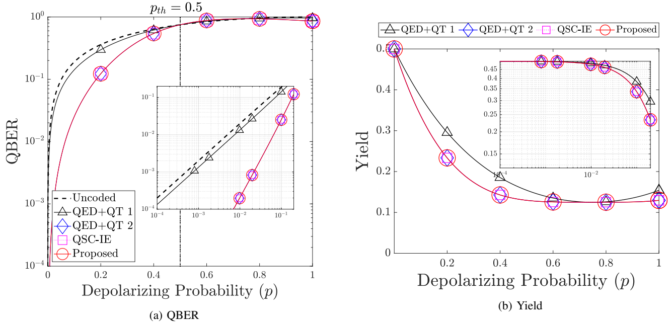
Fig. 8: The (a) QBER and the (b) yield of the proposed error-detection scheme in Fig. ?? compared to the existing schemes for mitigating the effect of quantum depolarizing channels. The uncoded QBER curve is given by \text{QBER} = 1 - (1-p)^2 = 2p - p^2 . The insets are the QBER and the yield in the logarithmic x axis.
