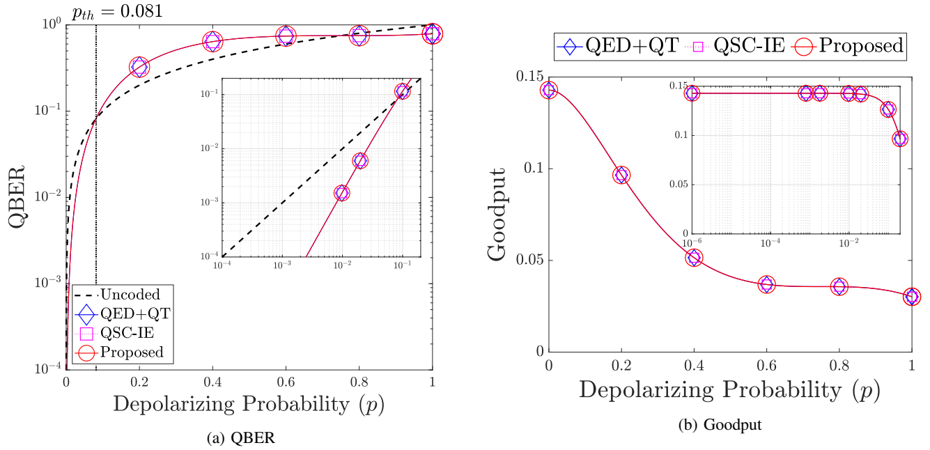
Fig. 12: The (a) QBER and the (b) goodput of our error-correction scheme proposed in Fig. ?? compared to the existing QSC-based scheme for mitigating the effect of quantum depolarizing channels. The insets are the QBER and the goodput in the logarithmic x axis.
