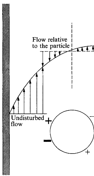
FIGURE 19. Cartoon showing the relative flow and pressure extrema around a neutrally buoyant particle in a Poiseuille flow. The particle is in a position marked in figure 17. R_p = 3.125 .
