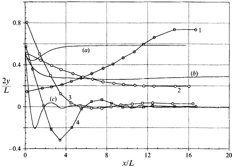
FIGURE 24. Migration of buoyant particles in a planar Poiseuille flow: comparison of our simulation with the experiment of Repetti & Leonard (1966). The centre is at y = 0 and the two walls are at y = \pm \frac{1}{2}L . Repetti & Leonard (downward flow): 1. Re_b = 412.3 , \kappa = 0.0951 , \delta\rho = 0.380\% ; 2. Re_b = 211.2 , \kappa = 0.0473 , \delta\rho = -0.091\% ; 3. Re_b = 408.5 , \kappa = 0.0948 , \delta\rho = -0.113\% ; 4. Re_b = 811.7 , \kappa = 0.0951 , \delta\rho = -0.322\% . Our simulation (upward flow) at Re_b = 120 , \kappa = 0.125 : (a) \delta\rho = -1\% , (b) \delta\rho = 1\% , (c) \delta\rho = 10\% .
