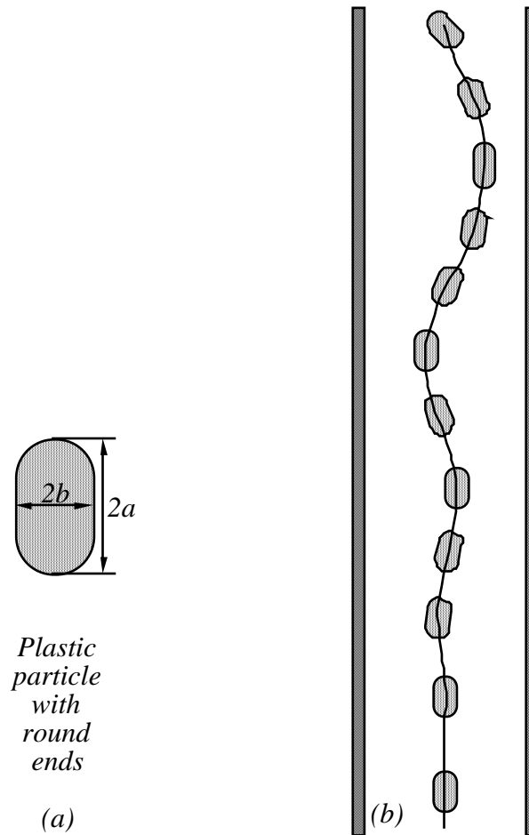
Figure 5. (a) A plastic long particle with round ends used in the experiment; (b) the long particle turns its longside parallel to the stream under the effects of lubrication in a Newtonian fluid when the channel is very narrow and the settling is very slow.
