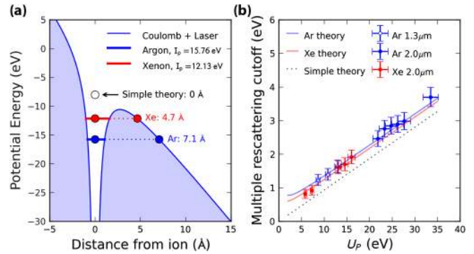
FIG. 4 (color online). (a) In the presence of a strong laser field ( 5 \times 10^{13} W/cm 2 ), the atomic Coulomb potential is deformed, enabling tunnel ionization. (b) By examining the classical equations of motion, we plot the theoretical cutoff between trajectories that revisit the ion once and those that rescatter several times (lines). If the tunnel distance is included, the theoretically predicted multiple rescattering cutoffs agree with the experimentally observed cutoffs (points). The experimental intensity was calibrated from the 2U_p cutoff. The error in the energy of the multiple rescattering cutoff was assumed to be 0.02 atomic units of momentum.
