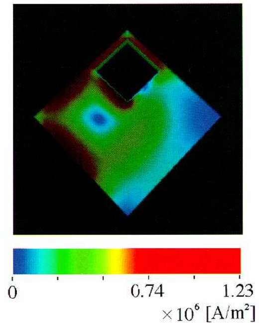
Figure 5 (b): Eddy current intensity distribution.
