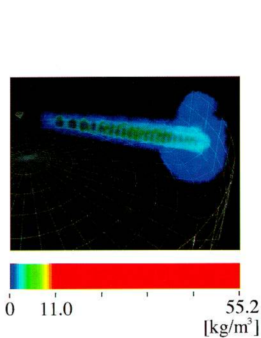
Figure 4 (c): Fuel density distribution.
