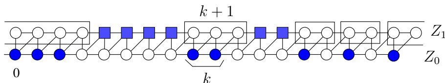
Figure 11: A block of k occupied positions in Z_0 determines k + 1 empty position on Z_1 (surrounded by rectangles). The little squares figure out the uncertain cells, that can not be determined just in view of the gas occupation in Z_0 .
