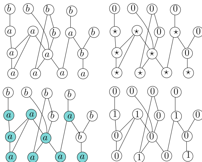
Figure 3: On the first column on top, a random coloring. Below, the family of DA derived from it. On the second column on top, the beginning of the computation of the gas occupation. “ \star ” stands for the places where the calculus X_x \leftarrow \prod_{c: \text{children of } x} (1 - X_c) must be done. Below, the gas occupation has been computed.
