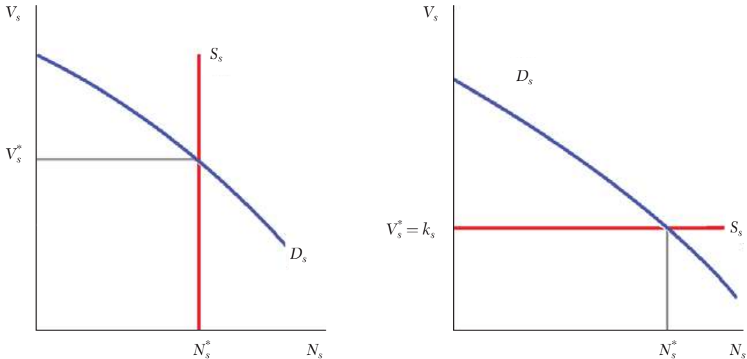
Figure 2. Equilibrium without (left) and with (right) Entry by Sellers
