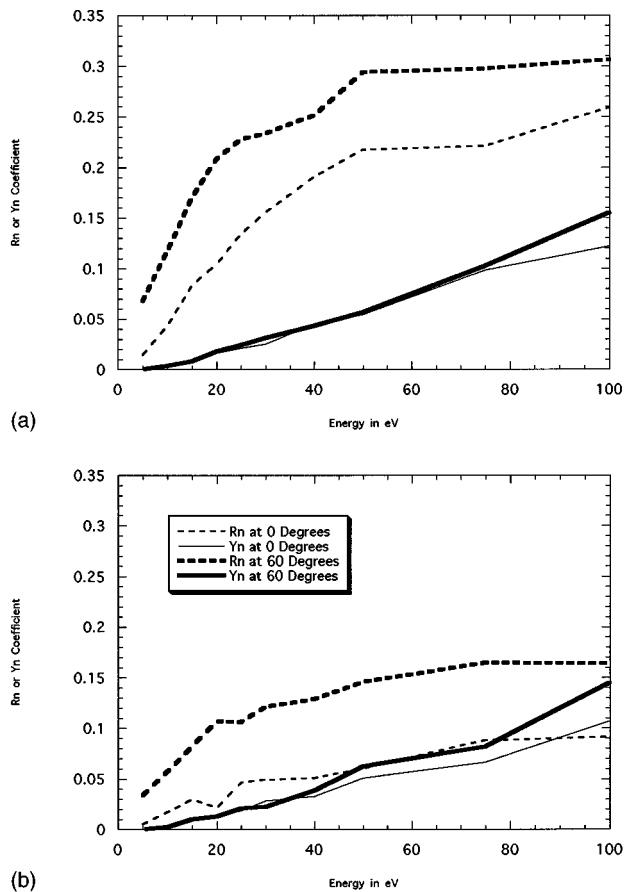
FIG. 3. Computer simulations of the reflection and sputtering yields for (A) Ar ions incident on Cu and (B) Cu ions incident on Cu.
