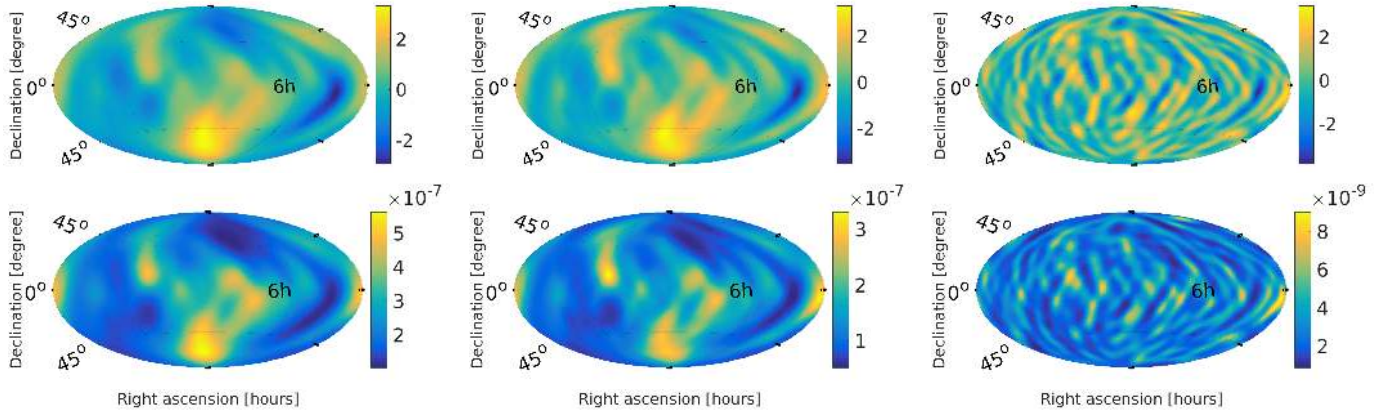
FIG. 1. All-sky radiometer maps for point-like sources showing SNR (top) and upper limits at 90% confidence on energy flux F_{\alpha, \theta_0} [ \text{erg cm}^{-2} \text{s}^{-1} \text{Hz}^{-1} ] (bottom) for three different power-law indices, \alpha = 0, 2/3 and 3 , from left to right, respectively. The p-values associated with the maximum SNR are (from left to right) p = 7\% , p = 12\% , p = 47\% (see Table I).
