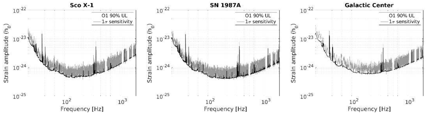
FIG. 4. Radiometer 90% upper limits on dimensionless strain amplitude ( h_0 ) as a function of frequency for Sco X-1 (left), SN1987A (middle) and the Galactic Center (right) for the O1 observing run (gray band) and standard deviation \sigma (black line). The large spikes correspond to harmonics of the 60 Hz power mains, calibration lines and suspension-wire resonances.
