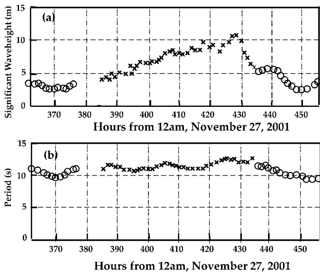
Fig. 14. (a). Significant waveheight measured with a long-range SeaSonde located at Winchester Bay, Oregon (crosses) and a standard-range SeaSonde at Washburn, Oregon (circles). (b). Wave periods measured with a long-range SeaSonde located at Winchester Bay, Oregon (crosses) and a standard-range SeaSonde at Washburn, Oregon (circles).
