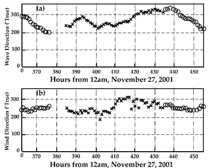
Fig. 15. (a). Wave directions measured with a long-range SeaSonde located at Winchester Bay, Oregon (crosses) and a standard-range SeaSonde at Washburn, Oregon (circles). The analysis assumes that waves of period greater than 6 s are onshore, as discussed in Section IV-A. (b). Wind directions measured with a long-range SeaSonde located at Winchester Bay, Oregon (crosses) and a standard-range SeaSonde at Washburn, Oregon (circles).
