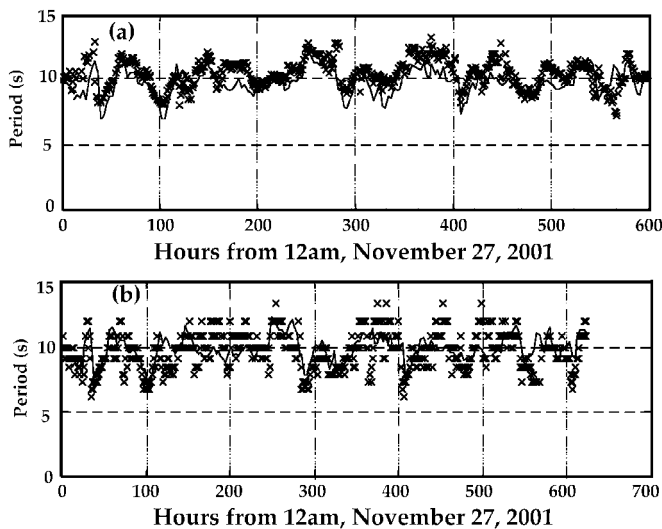
Fig. 5. Wave period comparison at BML. SeaSonde measurements of the period at the centroid of the spectrum (crosses) and from the S4 meter (continuous line). (a) SeaSonde results obtained using model-fitting. (b) SeaSonde results obtained using integral inversion.
