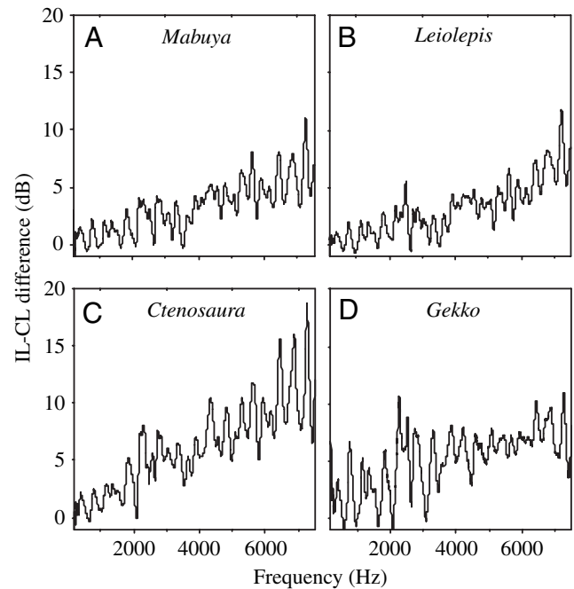
Fig. 4. Diffraction measured as ipsilateral–contralateral sound pressure difference measured by a probe microphone at the eardrum in Mabuya (A), Leiolepis (B), Ctenosaura (C) and Gekko (D).
