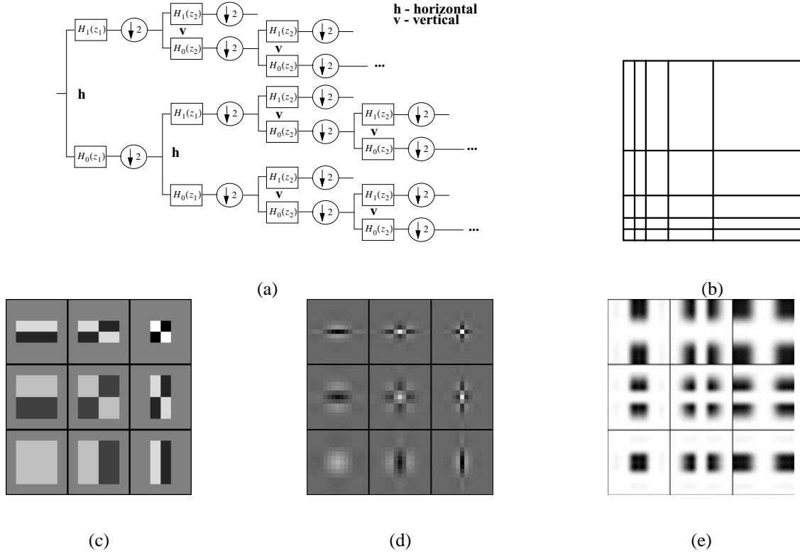
Fig. 4. The FSWT is anisotropic, as the number of 1-D transforms is not equal in the two directions. (a) An example of the transform scheme. Only 2 steps in each direction are shown. (b) The decomposition in frequency that corresponds to the construction in (a) with 4 steps in each direction. The anisotropic basis functions obtained from the (c) Haar and (d) biorthogonal "9-7" 1-D scaling and wavelet functions. (e) The corresponding Fourier transform of the basis functions obtained from the "9-7" 1-D filters.
