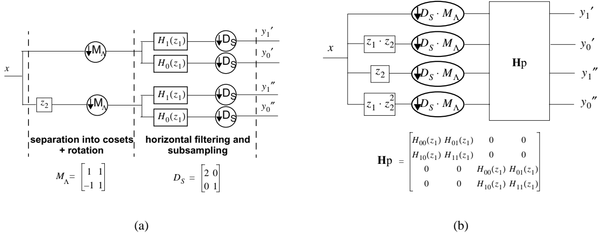
Fig. 12. (a) The 2-D two-channel filter-bank applied in the example shown in Fig. 9(a). Filtering and subsampling are applied in 2 cosets separately. (b) Equivalent polyphase representation contains 4 components. The polyphase transform \mathbf{H}_p is block-diagonal.
