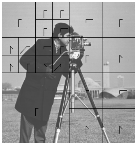
Fig. 15. The transform directions are adapted to the dominant directions in each segment of the image Cameraman shown in Figure 14(a).
