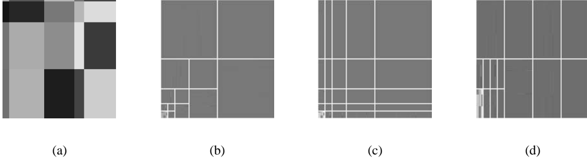
Fig. 3. (a) An image from the class \text{Mondrian}(k_1, k_2) . This class is inspired by the painting style established by Piet Mondrian (1872 - 1944). The image is transformed by the three transforms: (b) standard WT, (c) FSWT, (d) AWT(2,1) with 1-D wavelet filters having enough vanishing moments.
