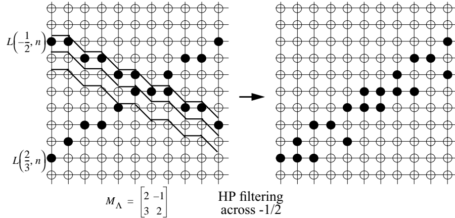
Fig. 7. A 1-D WT is applied on an image from the class S\text{-Mondrian}(M(-1/2, 2/3), 1, 1) along the digital lines L(-1/2, n) . The HP filtering annihilates the digital line with the slope -1/2 . However, the nonzero coefficients produced by the other line with the slope 2/3 are not aligned in the digital lines L(2/3, n) . This is called directional interaction . Although the transform along digital lines is efficient when applied in oversampled schemes, it fails to provide a systematic subsampling method when critical sampling is enforced.
