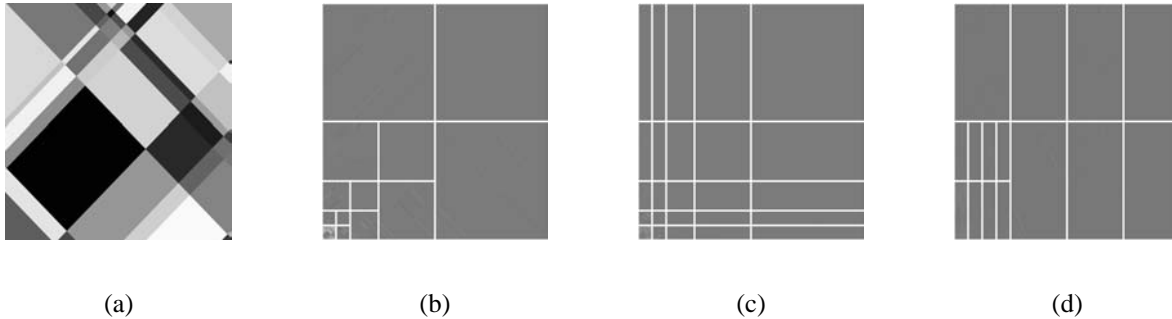
Fig. 6. (a) An example of an image from the class S\text{-Mondrian}(\mathbf{M}(r_1, r_2), k_1, k_2) , for \mathbf{M} = [\mathbf{v}_1, \mathbf{v}_2]^T , where \mathbf{v}_1 = [1, 1] and \mathbf{v}_2 = [-1, 1] . The image is transformed using (b) S-WT, (c) S-FSWT, and (d) S-AWT( \mathbf{M}_\Lambda, 2, 1 ) (directionlets), where all the transforms are built on the lattice \Lambda determined by the generator matrix \mathbf{M}_\Lambda = \mathbf{M}(r_1, r_2) .
