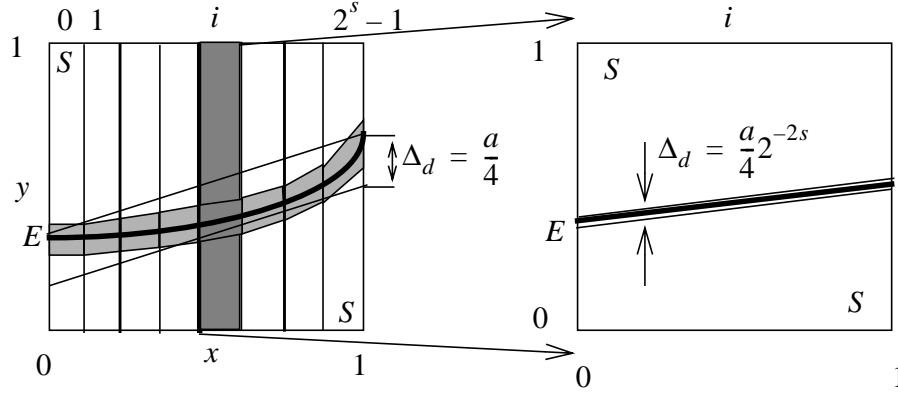
Fig. 17. Anisotropic segmentation partitions the unit square into 2^s equally wide vertical strips. After rescaling, the curvature parameter a (related to the second derivative of the C^2 curve) is reduced in each segment by the factor 2^{2s} . Since there are 2^s segments that intersect the discontinuity, the total number of the E-type transform coefficients is reduced by 2^s . At the same time, the total number of the S-type coefficients is increased by the same factor.
