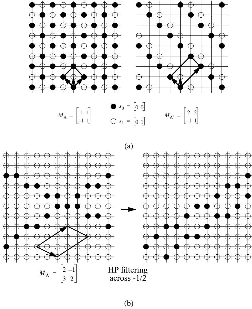
Fig. 9. (a) The lattice \Lambda is determined by the generator matrix M_\Lambda . 1-D Filtering is applied along the co-lines \{CL_{s_k}(r_1, n) : n \in \mathbb{Z}, k = 0, 1, \dots, |\det(M_\Lambda)| - 1\} , where the slope r_1 corresponds to the vector [1, 1] , that is, along 45^\circ . The pixels retained after the subsampling belong to the lattice \Lambda' \subset \Lambda determined by the generator matrix M_{\Lambda'} . Notice that filtering and subsampling are applied separately in two cosets, determined by the shift vectors s_0 and s_1 . (b) The nonzero pixels obtained after one step of the lattice-based filtering operation applied on the same example as in Fig. 7 are clustered in the digital lines with the slope 2/3 .
