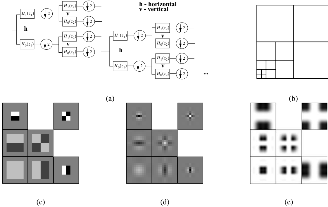
Fig. 1. The standard 2-D WT is isotropic. (a) The filtering and subsampling operations are applied equally in both directions at each scale of the transform. (b) The corresponding decomposition in frequency. The basis functions obtained in this way are isotropic at each scale as shown in (c) for Haar and in (d) for biorthogonal "9-7" 1-D scaling and wavelet functions. (e) The corresponding Fourier transforms of the basis functions obtained from the "9-7" 1-D filters.
