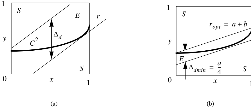
Fig. 16. The 2-D function f(x_1, x_2) is C^2 smooth on the unit square away from a C^2 discontinuity curve. The curve can be locally approximated by a quadratic polynomial y(x) = ax^2 + bx + c . The E-type transform coefficients intersect the curve and have a slower decay of magnitudes across scales than the S-type coefficients, which correspond to the smooth regions. (a) The S-AWT produces the E-type coefficients within the strip along the slope r . (b) The width of the strip \Delta_d is minimized for r = a + b .
