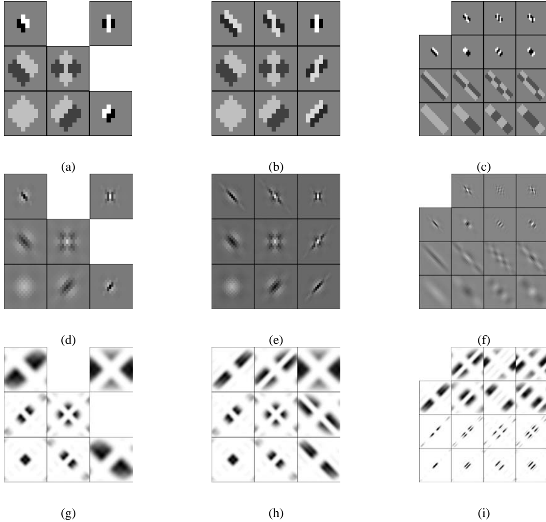
Fig. 10. The basis functions obtained by the skewed transforms using the Haar 1-D scaling and wavelet functions: (a) S-WT, (b) S-FSWT, (c) S-AWT( M_\Lambda, 2, 1 ) (directionlets). The same, but with the biorthogonal "9-7" 1-D scaling and wavelet functions: (d) S-WT, (e) S-FSWT, (f) S-AWT( M_\Lambda, 2, 1 ) (directionlets). In all cases M_\Lambda = [\mathbf{d}_1, \mathbf{d}_2]^T , where \mathbf{d}_1 = [1, 1] , and \mathbf{d}_2 = [-1, 1] . The DVMs are imposed along the vectors \mathbf{d}_1 and \mathbf{d}_2 , that is, along 45^\circ and -45^\circ . The corresponding Fourier transforms: (g) S-WT, (h) S-FSWT, (i) S-AWT( M_\Lambda, 2, 1 ) (directionlets).
