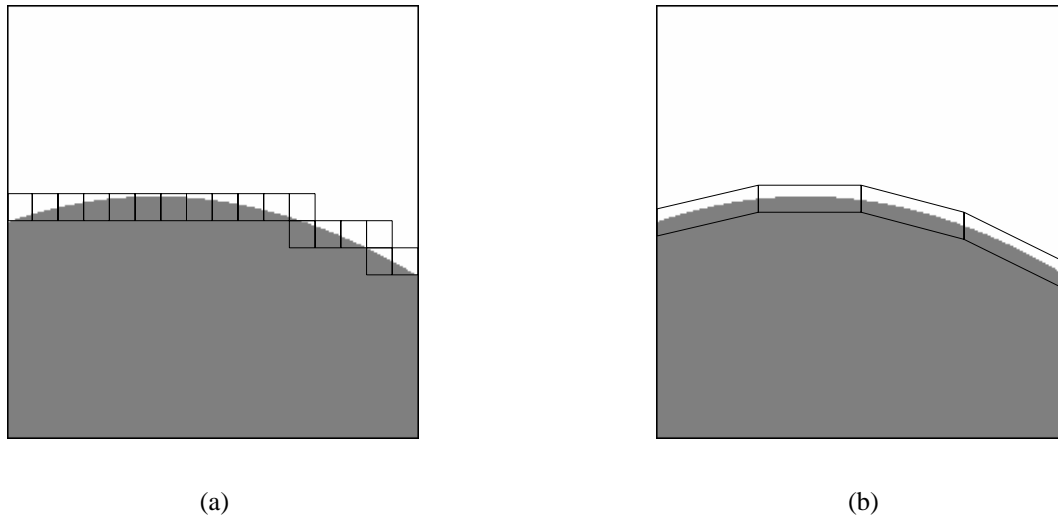
Fig. 2. A simple image with one discontinuity along a smooth curve is represented by the two types of basis functions: isotropic and anisotropic. The support of these basis functions is shown schematically as black rectangles. (a) Isotropic basis functions generate a large number of significant coefficients around the discontinuity. (b) Anisotropic basis functions trace the discontinuity line and produce just a few significant coefficients.
