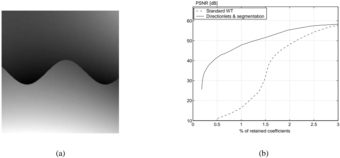
Fig. 13. An example of NLA of an image from the class C^2/C^2 . (a) An image from the class C^2/C^2 is approximated using the standard WT and the S-AWT( \Lambda, 2, 1 ) with spatial segmentation. (b) The MSE expressed in terms of PSNR is significantly reduced in the case of the S-AWT( \Lambda, 2, 1 ).
