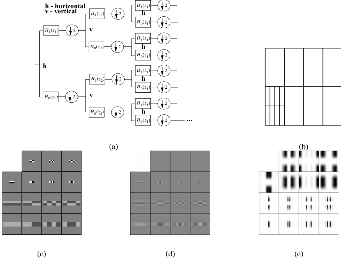
Fig. 5. The AWT allows for anisotropic iteration of the filtering and subsampling applied on the LP, similarly as in the standard WT. Although this transform does not improve approximation of the class \text{Mondrian}(k_1, k_2) , it provides an efficient approximation tool for more general classes of images (Section IV). (a) The filtering scheme for the AWT(2,1), where one step of iteration is shown. (b) The decomposition in frequency. The basis functions obtained from the (c) Haar and (d) biorthogonal "9-7" 1-D scaling and wavelet functions. (e) The corresponding Fourier transform of the basis functions obtained from the "9-7" 1-D filters.
