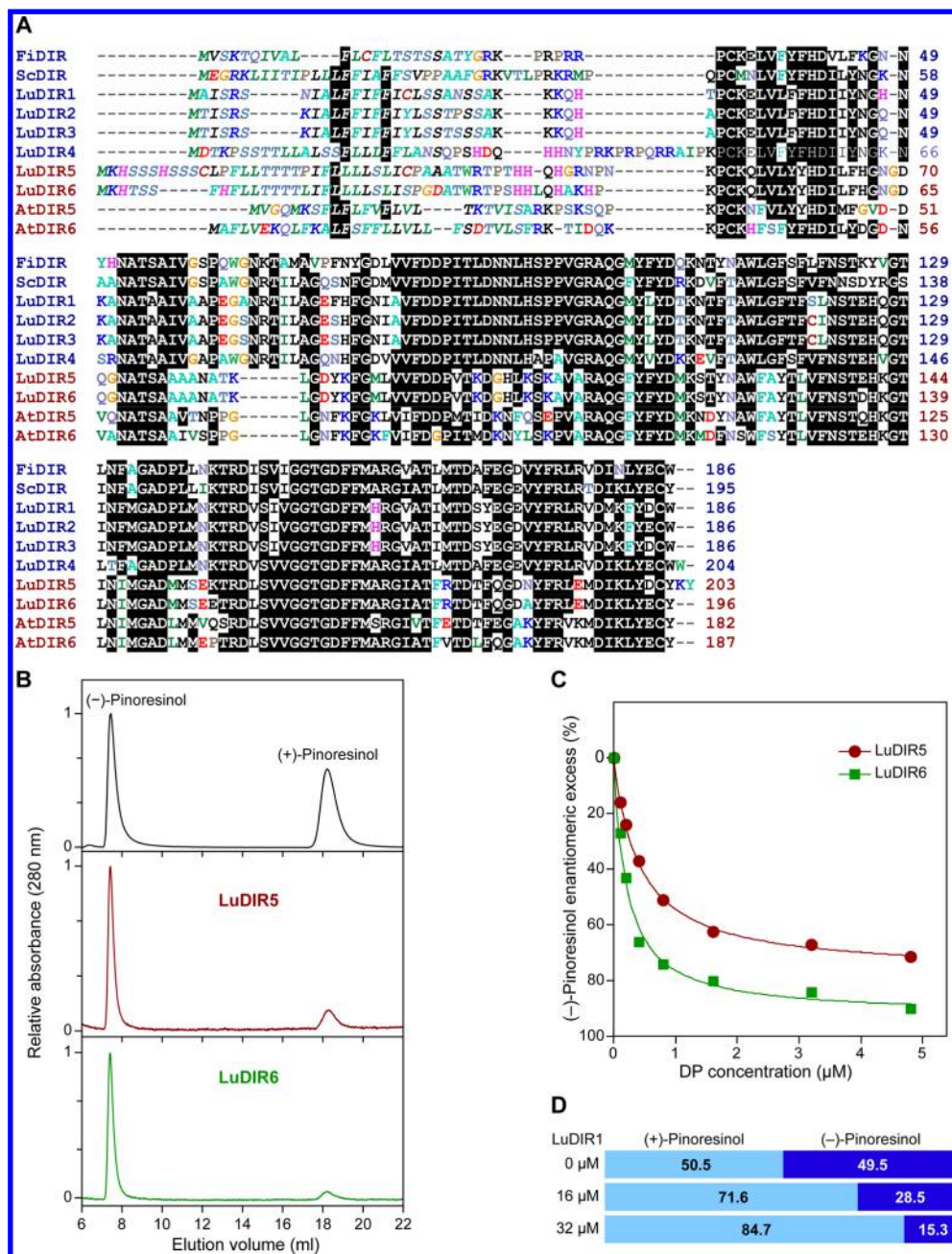
Figure 2. (A) Amino acid sequence comparison of LuDIR homologues (LuDIR1–LuDIR6) with (+)-pinoresinol-forming DPs (FiDIR and ScDIR) and (–)-pinoresinol-forming DPs (AtDIR5 and AtDIR6). Signal peptides were predicted with the SignalP 4.1 Server and are denoted in italic characters. At, Arabidopsis thaliana ; Fi, Forsythia intermedia ; Lu, Linum usitatissimum ; Sc, Schizandra chinensis . (B–D) Differential stereoselectivity of distinct recombinant flax DPs. (B) Chiral HPLC analyses of authentic racemic (±)-pinoresinols (9a/9b, top panel), and pinoresinol (9a/9b) products formed by recombinant LuDIR5 (4.8 μM, middle panel) and LuDIR6 (4.8 μM, bottom panel), respectively. (C) Enantiomeric excess (ee) of (–)-pinoresinol (9b) formation at various concentrations of recombinant LuDIR5 and LuDIR6. (D) Ratios of (+)- and (–)-pinoresinols (9a and 9b) formed using different concentrations of recombinant LuDIR1. In (C) and (D), each data point corresponds to a single independent measurement for each concentration tested. The experiments were repeated 4 times with similar results.
