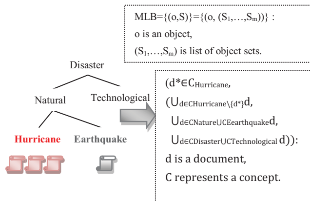
Figure 4. MLB constraints from partial hierarchy
